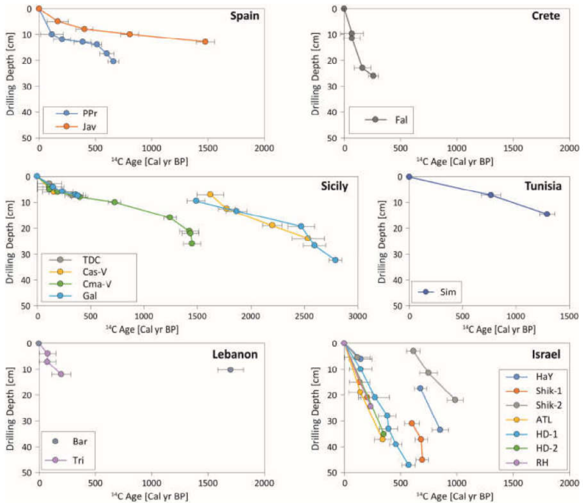
561 562 Fig. 8. Vertical growth rates (drilling depth vs. ^{14}\text{C} age) of vermetid reefs along a Mediterranean 563 west-east transect. All data, except from Israel (Sisma-Ventura, 2014), are newly obtained and 564 presented for the first time in the current paper. The vermetids of the western basin show older 565 ages, but relatively low rates, compared to the much younger ages and higher growth rates in the 566 eastern basin.
