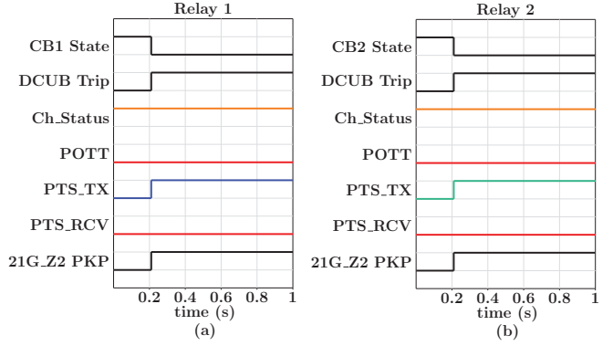
Fig. 19. DCUB protection signals and circuit breakers state of (a) Relay 1 and CB1 and (b) Relay 2 and CB2 considering the DDoS attack on the communication channel.
