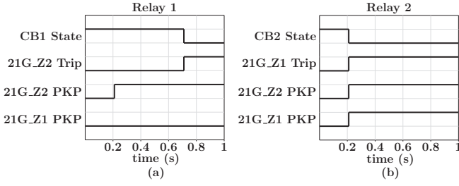
Fig. 8. Step-distance relay signals and circuit breakers state of (a) Relay 1 and CB1 and (b) Relay 2 and CB2.
