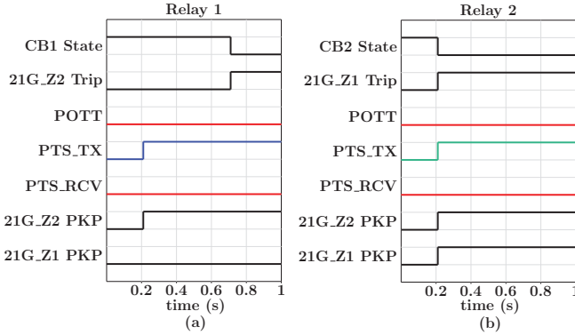
Fig. 13. POTT protection signals and circuit breakers state of (a) Relay 1 and CB1 and (b) Relay 2 and CB2 considering the DDoS attack.
