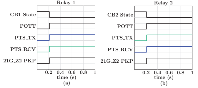
Fig. 10. POTT protection signals and circuit breakers state of (a) Relay 1 and CB1 and (b) Relay 2 and CB2.
