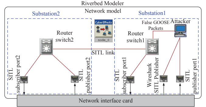
Fig. 20. The FDI attack implemented using Wireshark tool and Riverbed Modeler.
