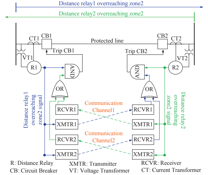
Fig. 2. The POTT protection scheme with communication channel redundancy.
