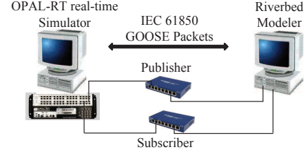
Fig. 4. Schematic representation of the co-simulation platform.
