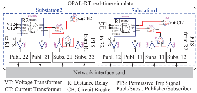
Fig. 15. Schematic representation of the implementation of the POTT protection with communication redundancy in OPAL-RT real-time simulator.
