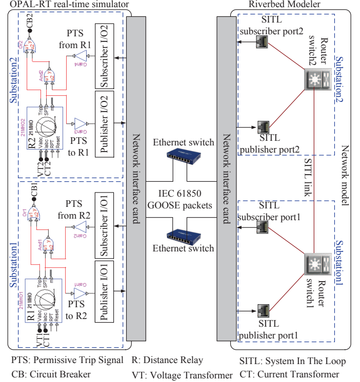
Fig. 5. Schematic representation of the implementation of the benchmark test system in the cosimulator.
