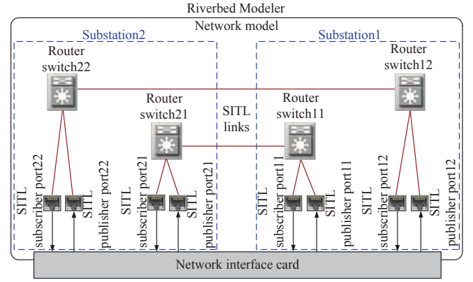
Fig. 14. The implementation of the communication channel redundancy between the relays in Riverbed Modeler.
