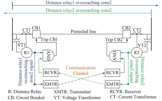
Fig. 1. The POTT protection scheme.
