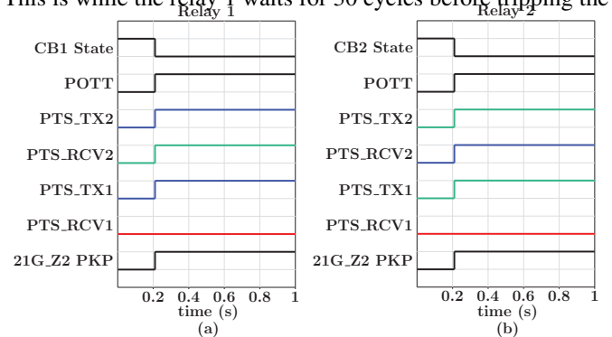
Fig. 16. POTT protection with communication channel redundancy signals and circuit breakers state considering the DDoS attack on the communication channel1 (a) Relay 1 and CB1, (b) Relay 2 and CB2.
