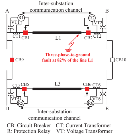
Fig. 7. Part of the IEEE PSRC D6 benchmark test system illustrating a permanent three-phase-to-ground fault on line L1.
