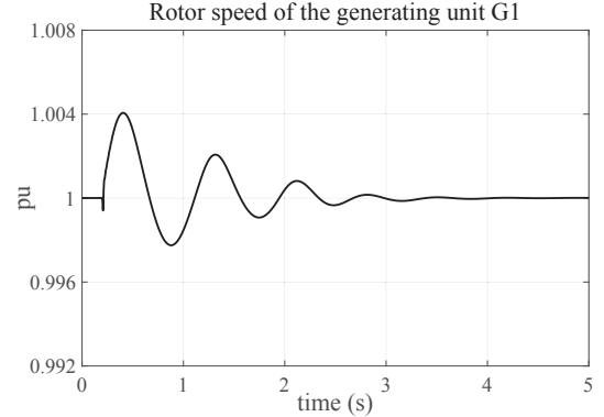
Fig. 11. The rotor speed of the generating unit G1 when the permanent three-phase-to-ground fault at 82% of the line L1 is cleared instantaneously. circuit breakers CB1 and CB2 disconnects the transmission line L1 from the buses A and B and instantaneously clears the faults. As illustrated in Fig. 11 for the generating unit G1, the generators' rotor speed remains stable in this case.
