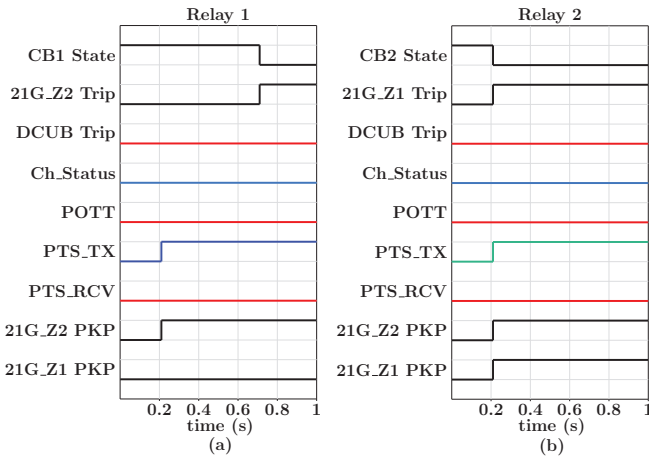
Fig. 21. DCUB protection signals and circuit breakers state of (a) Relay 1 and CB1 and (b) Relay 2 and CB2 considering the FDI attack on the communication channel.
