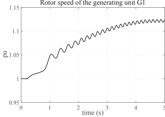
Fig. 9. The rotor speed of the generating unit G1 when the permanent three-phase-to-ground fault at 82% of the line L1 is cleared after 30 cycles.
