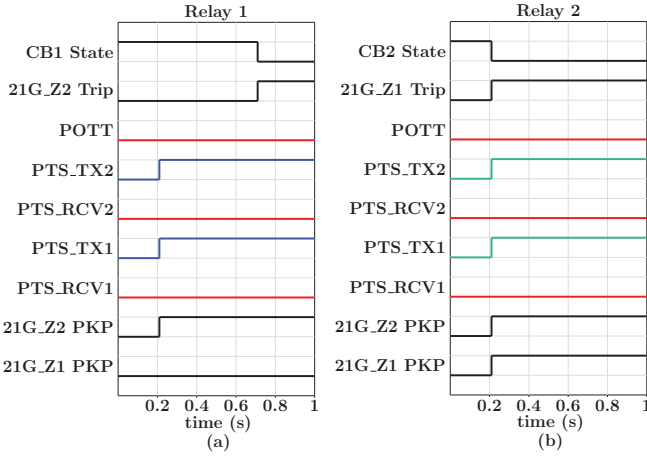
Fig. 17. POTT protection with communication channel redundancy signals and circuit breakers state of (a) Relay 1 and CB1 and (b) Relay 2 and CB2 considering the DDoS attack on both communication channels.
