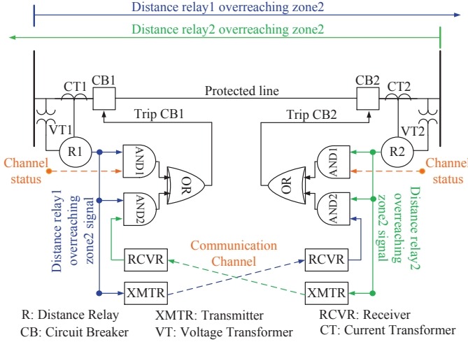
Fig. 3. The DCUB protection scheme.
