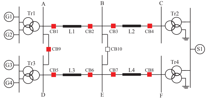
Fig. 6. The IEEE PSRC D6 benchmark test system.
