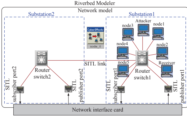
Fig. 12. The DDoS attack implemented in Riverbed Modeler on the communication channel between distance relays.
