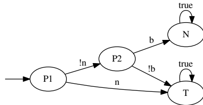
Fig. 2: A monitor for LTL formula \phi_6 := GF r \vee (\neg n \rightarrow X\neg b) . Each transition is labeled with a propositional formula denoting a set of satisfying states. For example, “!n” denotes \{\emptyset, \{r\}, \{b\}, \{r, b\}\} and “true” denotes all states.
