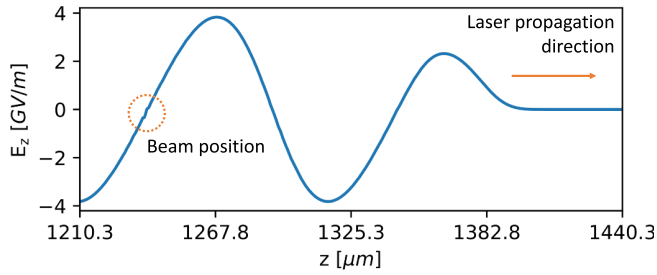
Fig. 15.2. On-axis longitudinal electric field after 1.2 mm of propagation in the plasma, with the electron beam placed at the zero crossing (case with \Delta\xi = 0 ).
