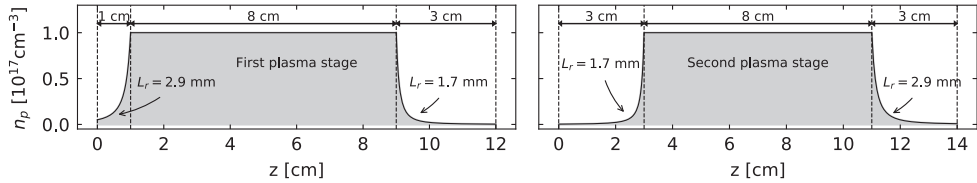
Fig. 23.33. On-axis density profile of the two plasma stages.
