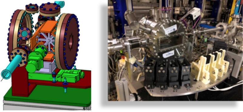
Fig. 32.23. The SPARC_LAB experimental apparatus (right) and conceptual drawing (left), as seen after its installation in 2018.
