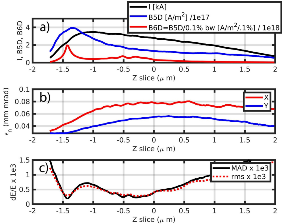
Fig. 23.11. Slice analysis with a slice thickness of 0.1 μm. The longitudinal axis corresponds to the slice position with respect to beam centre of mass. a) Current (black), 5D brightness B_{5D} \equiv 2I/(\pi^2 \epsilon_{nx} \times \epsilon_{ny}) (blue), and 6D brightness B_{6D} \equiv B_{5D}/(\sigma_E/E/10^3) (red). b) Emittances in the x (red) and y (blue) directions. c) Energy spread using the RMS estimator (red, dashed) or the Mean Absolute Deviation robust indicator (black) (reprinted from [594] with permission, copyright IOP Publishing).
