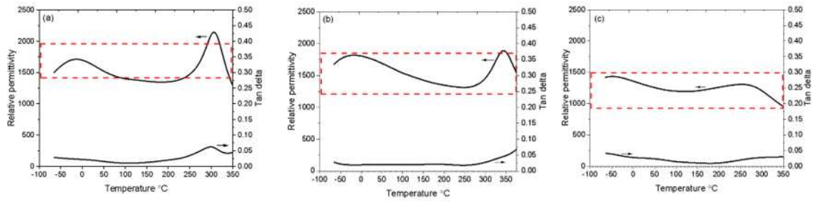
Figure 7. Comparisons of the 1 kHz relative permittivity, highlighting the stability in \epsilon_r values from -65\text{ }^\circ\text{C} to \geq 300\text{ }^\circ\text{C} in \text{Sr}_{2-2z}\text{Ca}_z\text{Y}_z\text{NaNb}_{5-z}\text{Zr}_2\text{O}_{15} : (a) z = 0 ; (b) z = 0.025 ; (c) z = 0.05 . The dashed outline indicates the \pm 15\% limits required by the EIA. Dielectric loss tangent plots are also shown.
