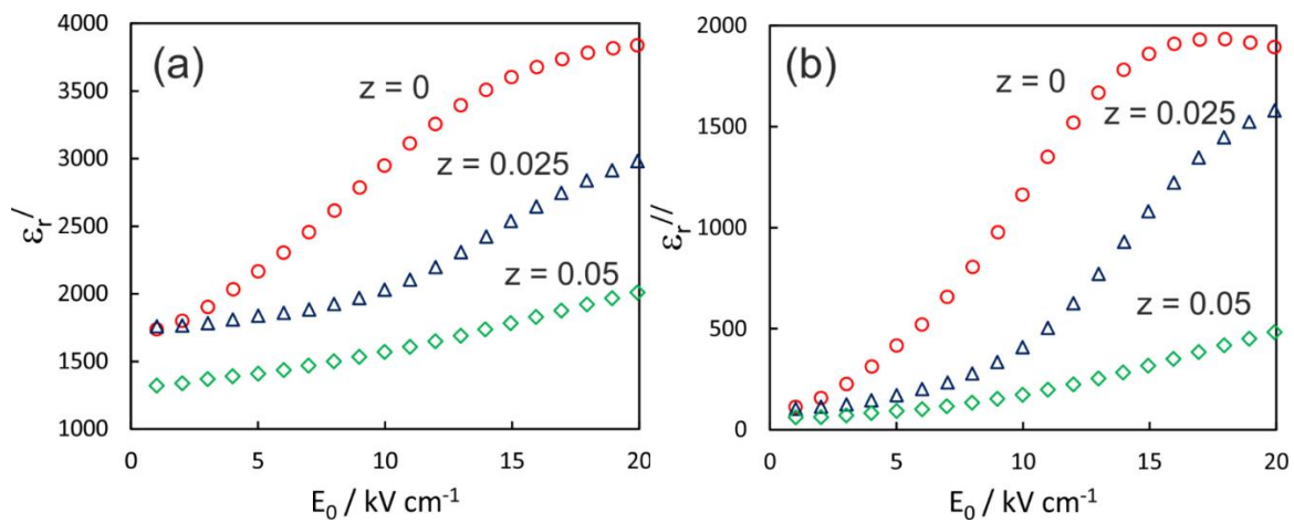
Figure 9. Variations in (a) real and (b) imaginary parts of relative permittivity as a function of increasing electric field amplitude
