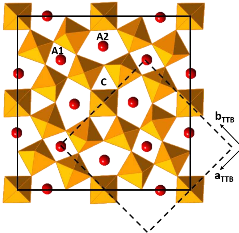
Figure 1 Pseudocubic tetragonal primary cell of tungsten bronze structure (dashed lines) viewed along the [001] direction and its spatial relationship to a larger orthorhombic unit cell arising from by a superstructure (solid lines; after Ref 20]. In \text{Sr}_4\text{Na}_2\text{Nb}_{10}\text{O}_{30} \text{Sr}^{2+} and \text{Na}^+ ions are distributed over the A1 and A2 sites (red) formed by corner sharing \text{NbO}_6 octahedra (orange).
