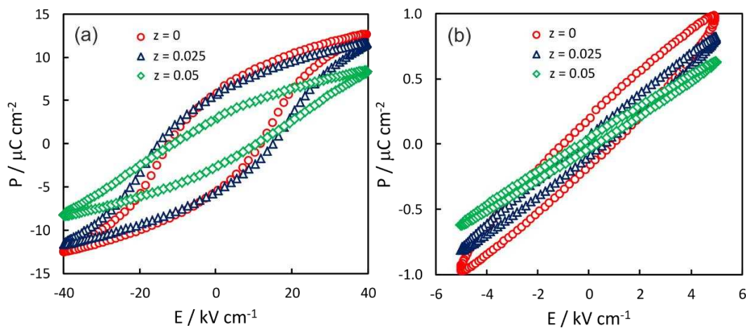
Figure 8 Comparison of P-E loops for (a) E_{\text{max}} = 40 \text{ kV cm}^{-1} and (b) E_{\text{max}} = 5 \text{ kV cm}^{-1} .
