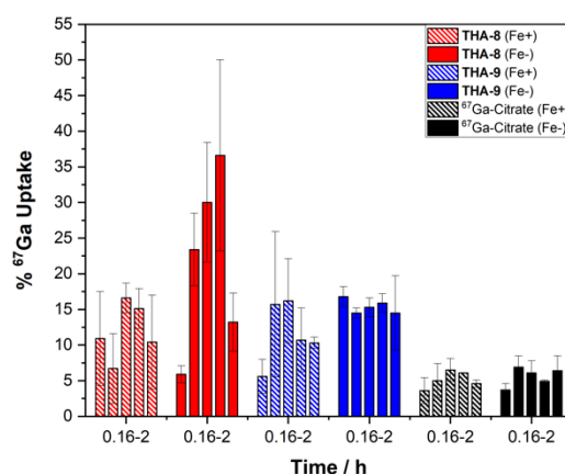
Figure 25. Results of THA-8 and THA-9 radiochemical uptake studies in E. coli for iron-sufficient (striped bars) and iron-limited conditions (solid bars). ^{67}\text{Ga} citrate is included for comparison. [48] Measurements were taken at 0.16 h, 0.33 h, 0.50 h, 1 h and 2 h timepoints.
