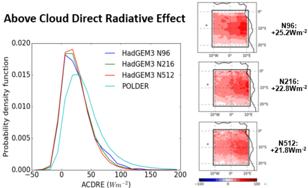
1335 Figure 18: Showing the above cloud direct radiative effect diagnosed from the Unified model (N96, N216 and N512 resolution, approximately 140, 60 and 25 km respectively) over the area shown in the panels in the right-hand column. The probability density function of the above cloud direct radiative effect is also shown from POLDER after (Peers et al. , 2016). The intercomparison is for August-September 2006 and model data is matched to instantaneous POLDER retrievals.
