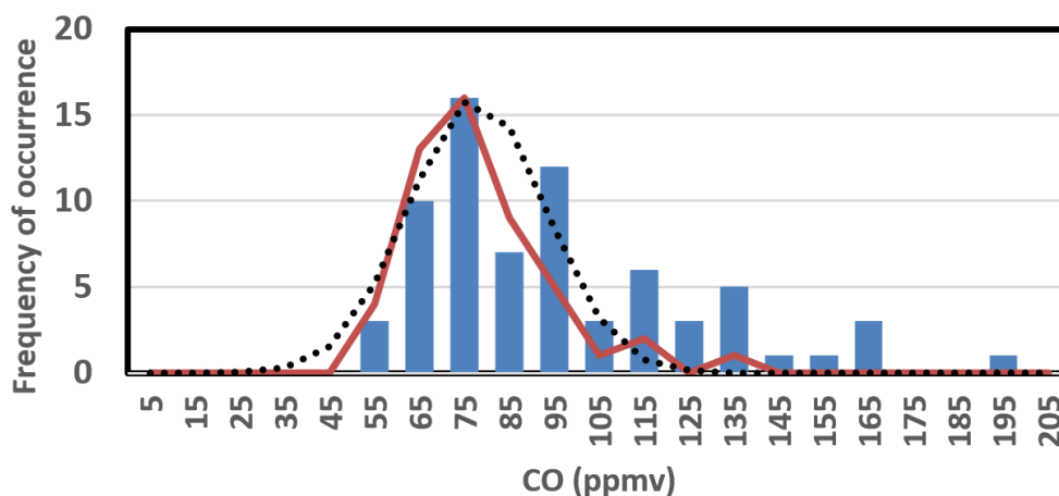
1330 Figure 17: The carbon monoxide (CO) concentrations for precipitating (red curve) and non-precipitating days (blue bars). A Gaussian fit to the non-precipitating data is shown by the dotted lines.
