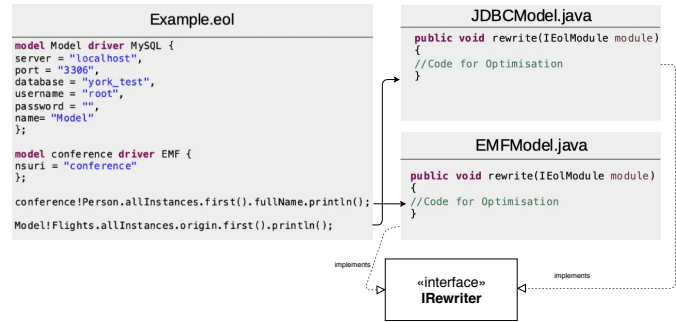
Figure 3: IRewriter interface architecture
