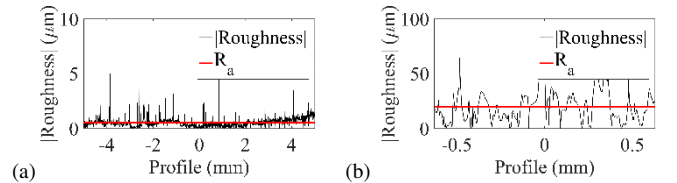
Fig. 3. Roughness profile of (a) conventional and (b) additively manufactured rods used to calculate R_a values.
