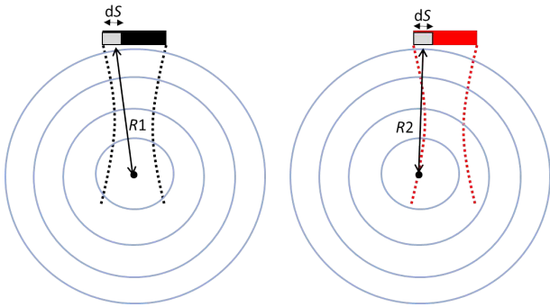
Fig. 2. Schematic illustration of echo reception by a single-element transducer. Depending on the location of the scatterer, the integrated waveform projected onto the receive aperture can be different. The rings indicate the wavefronts. R1 and R2 are the distances between the scatterer (black point) and the receive sub-aperture dS .
