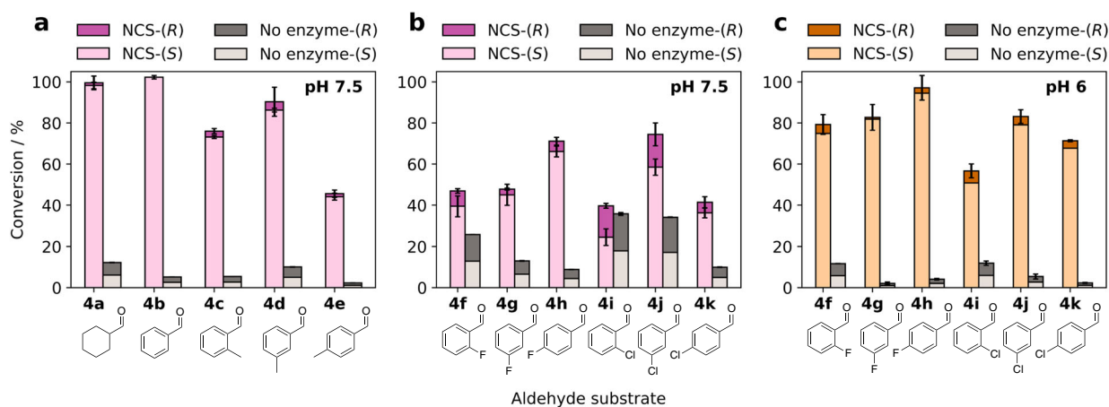
Fig. 4 Conversions (determined against product standards) and enantiomeric excesses of products generated by a M97V- \Delta 29T /NCS-catalysed reaction between dopamine and a variety of aldehyde derivatives. Reactions were performed using 0.5 \text{ mg mL}^{-1} final concentration of enzyme for 24 h. a Reactions between dopamine ( 1 ) and 4a–e at pH 7.5. b Reactions between dopamine ( 1 ) and 4f–k at pH 7.5. c Reactions between dopamine ( 1 ) and 4f–k at pH 6. Reactions were performed in triplicate and the error bars given are the standard deviations.
