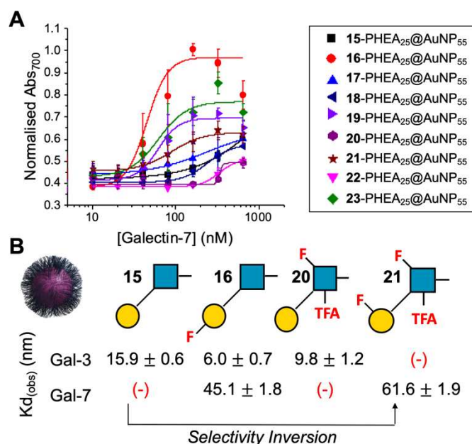
Figure 5. Galectin-7 binding to the F-glyconanoparticle library. A) Dose-response curve for the AuNP aggregation assay; B) Summary of apparent K_d (nM) for selected glycans showing the fine-tuning and selectivity inversion. (-) = no binding
