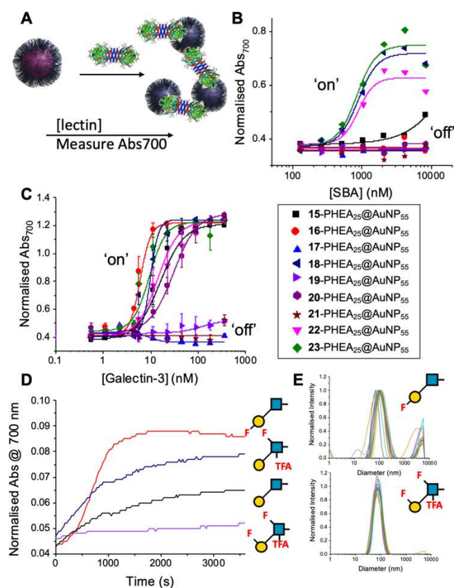
Figure 3. Screening of lectin/F-GlycoNP binding. A) Schematic of aggregation assay; B) Dose response to Soy Bean Agglutinin
