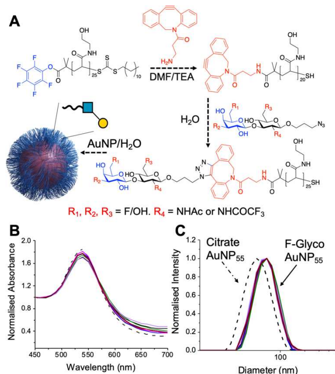
Figure 2. Nanoparticle synthesis and characterization. A) Synthetic route to conjugate fluoro-glycans onto nanoparticles; B) UV-Vis traces of all nanoparticles showing colloidal stability; C) Dynamic light scattering (DLS) of all nanoparticles showing size increase upon polymer coating.
