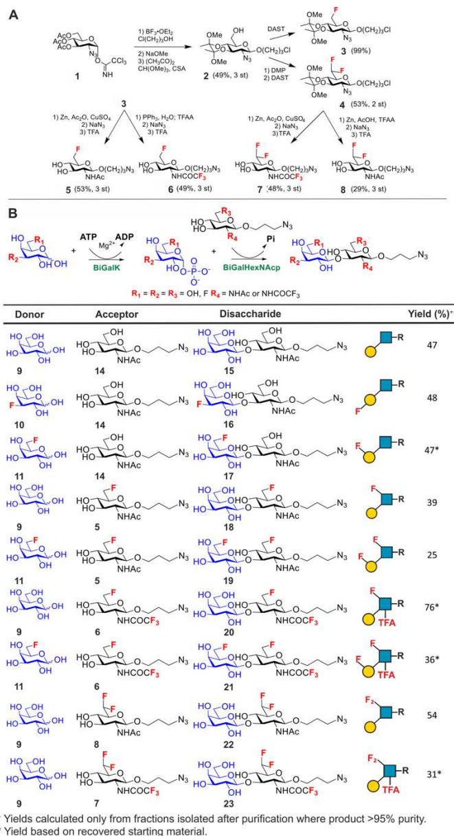
Figure 1. A. Chemical syntheses of fluorinated acceptors. B) Fluorinated lacto- N -biose analogues prepared using a chemoenzymatic strategy with BiGalK and BiGalHexNAcP. TFA = trifluoroacetyl.
