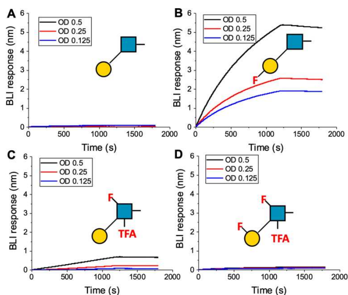
Figure 4. Biolayer interferometry analysis of binding of AuNPs to Galectin-3. A) Lacto- N -biose ( 15 ); B) 3FGal- \beta (1,3)-GlcNAc ( 16 ); C) Gal- \beta (1,3)-6FGlcNTFA, ( 20 ); D) 6FGal- \beta (1,3)-6FGlcNTFA, ( 21 ).
