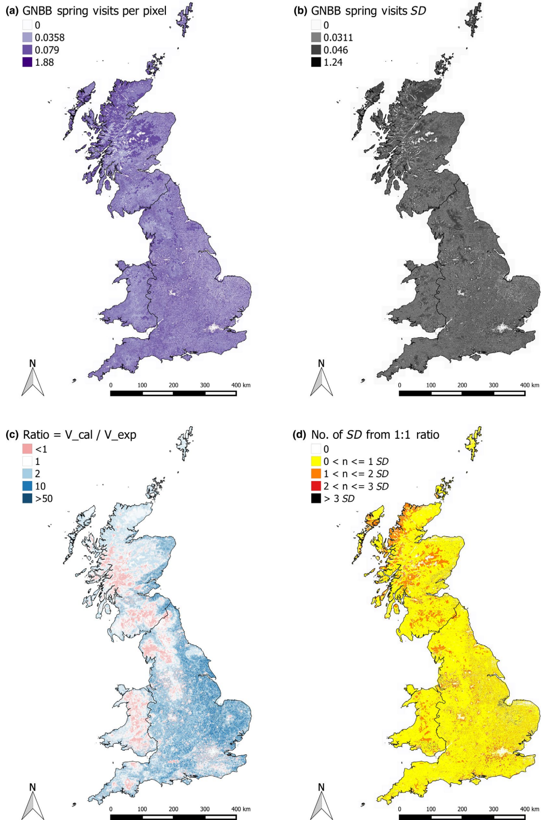
FIGURE 7 (a) Model predictions for Ground Nesting Bumblebee spring visitation rate across Great Britain using attractivenness scores obtained via calibration Method 1. (b) SD of model predictions shown in (a). (c) Ratio between (a) and model predictions using original expert opinion attractivenness scores. (d) Number of SDs of ratio away from 1:1. Figures S4, S5 and S6 show corresponding maps for the other pollinator guilds
