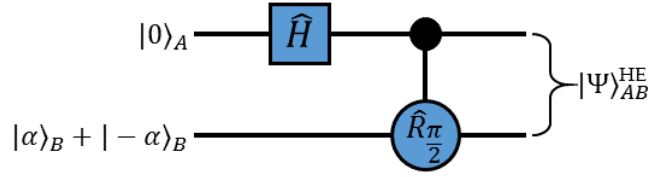
Figure 2: A quantum circuit which could be used to prepare the initial hybrid entangled states ( |\Psi\rangle_{AB}^{HE} and |\Psi\rangle_{CD}^{HE} ), as given in Eq. 3) for our proposed entanglement swapping protocol, using a Hadamard gate ( \hat{H} ) and a controlled \frac{\pi}{2} rotation gate ( \hat{R}_{\frac{\pi}{2}} ).
