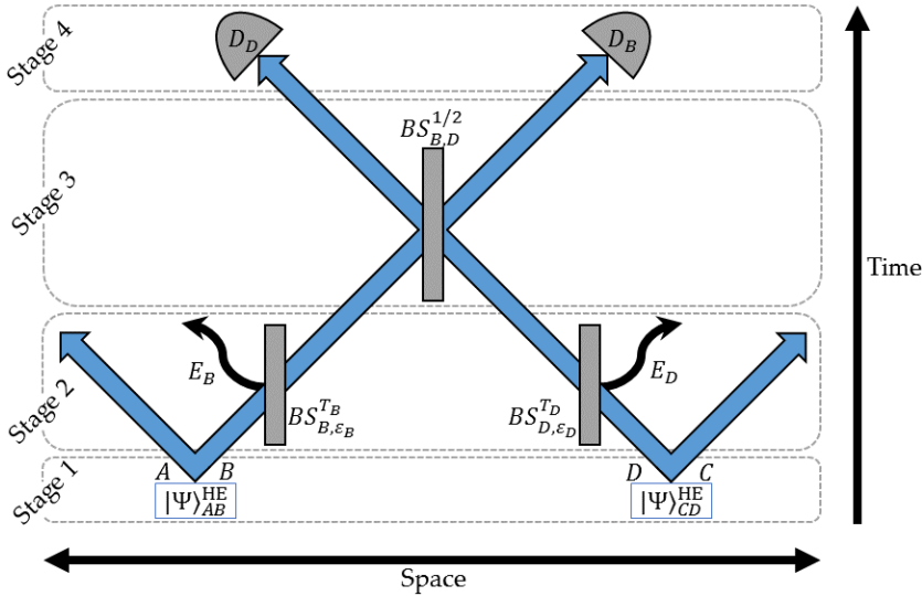
Figure 1: Schematic to represent the six channel system (in which the initial hybrid entangled states are denoted as |\Psi_{AB}^{HE}\rangle and |\Psi_{CD}^{HE}\rangle ) undergoing entanglement swapping. Modes A and C are the discrete variable post-entangled modes, and B and D are the propagating continuous variable modes. Losses are modelled through leakage of modes B and D into modes E_B and E_D respectively. The lossy modes B and D then meet at a 50:50 beam-splitter ( BS_{B,D}^{1/2} ) before subsequently being measured via a projective vacuum measurement and balanced homodyne detection ( D_B and D_D , respectively).
