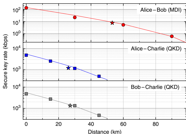
Fig. 3 Secure key rates vs. distance. MDI-QKD (top diagram) and QKD (centre and bottom diagrams) secure key rates for a Z (X) basis probability equal to 80% (20%) and a security parameter e_{\text{sec}} \lesssim 10^{-10} are shown as a function of distance. Because the reconfigurable scheme is symmetrically deployed, the distance between Alice and Bob (top) is approximately twice the distance between Alice and Charlie (centre) and Bob and Charlie (bottom). All the distances have been calculated assuming 0.2 dB/km attenuation on the channel, except for the data points indicated by stars, where a real fibre was used. The projected time to attain the shown key rates is 25 h of which 3 min are spent on QKD and the rest on MDI-QKD, to balance their key rates. The fitting lines are the result of a numerical simulation with the parameters mentioned above and the following additional ones: Charlie’s insertion loss, 1.1 dB; detectors’ efficiency and temperature, 20% and 0°, respectively; afterpulsing, 4%; dark count probability per gate, 1.6 \times 10^{-5} ; error correction coefficient, 1.16
