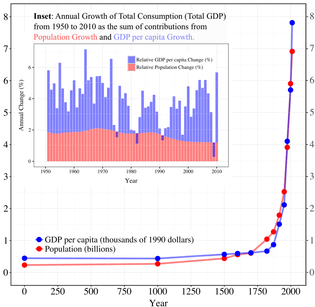
Population and GDP per capita (in the main graph) from year 1 to 2010 AD. The total human impact is their product.
