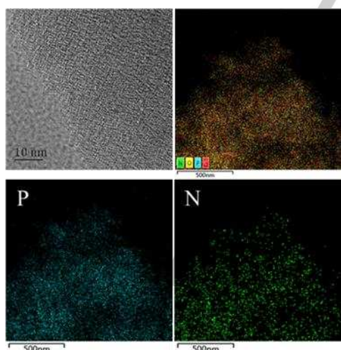
Figure 2. High TEM image of the P-C-N-5-800 catalyst and elemental mapping of the P-C-N-5-800 catalyst.
