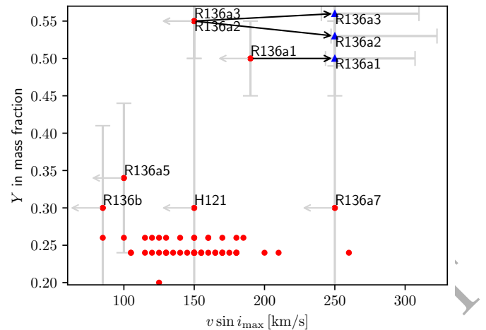
Figure 7. Surface helium abundances versus upper limits of the projected rotation (red dots and arrows pointing to the left). There is no clear correlation between v \sin i_{\text{max}} and Y . Blue triangles indicated the most probable current day rotation rates for the three WNH stars, which largely excludes v_{\text{rot}} < 250 \text{ km/s} .
