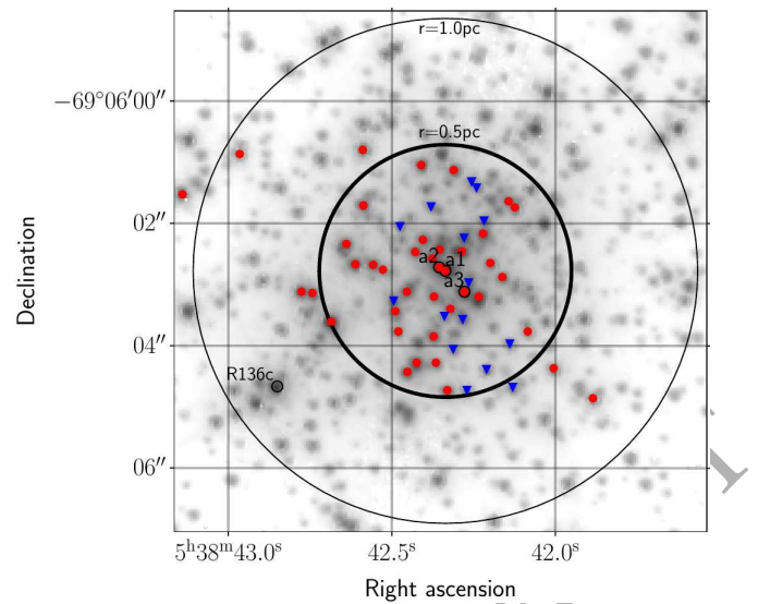
Figure 11. Spatial distribution of our targets in R136. Stars indicated by a red dot likely belong to a younger population while blue triangles to an older ( \gtrsim 2.5 Myr). The position of older and younger stars are randomly distributed. Black bold solid circle of radius 0.5 parsec and black solid circle of radius 1.0 parsec are centred on R136a1. The background image was taken with HST/WFC3 using the F555W filter.
