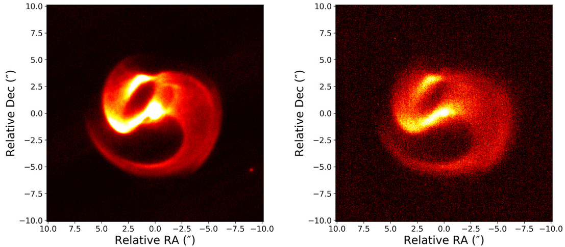
Figure 1. Reduced 2018 epoch images taken with the J8.9 filter (left) and Q3 filter (right). The normalized pixel values were stretched from 0 to 0.03 in J8.9 and to 0.5 in Q3 on a linear scale. The faint background star used for plate scale calibration, 2MASS J16004953-5142506, is just visible to the south-west of the plume near the edge of the field in the J8.9 data.
