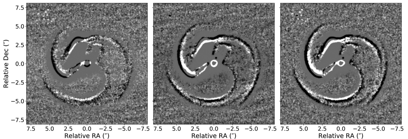
Figure B1. High-pass filtered difference images in which newer epochs have been subtracted from older. Data from 2016 and 2017 (left), 2017 and 2018 (middle), and 2016 and 2018 (right). Negative images (black) always lie exterior to positive ones (white) implying the expansion of the dust plume is clearly visible across all combinations.
