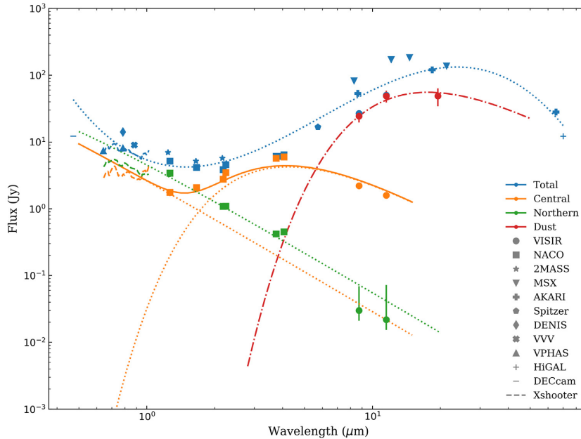
Figure 3. The optical and infrared SED of Apep’s components (central binary, northern companion, and dust plume) dereddened with A_v = 11.4 (Callingham et al. 2019; Mathis 1990). The SEDs of the Apep system and calibrator stars listed in Table 1 are quoted from the DECcam (g) (Abbott et al. 2018), VPHAS + (r, i) (Drew et al. 2014), DENIS (i) (Epchtein et al. 1999), VVV (Z) (Minniti et al. 2010), 2MASS (J, H, Ks) (Skrutskie et al. 2006), IRAC (5.8-micron) (Werner et al. 2004), MSX (A, C, D, E) (Price et al. 2001), AKARI (S9W, L18W, N60) (Doi et al. 2015) and Hi-GAL (70-micron) (Molinari et al. 2016) surveys and the calibrated XSHOOTER spectrum (moving average with 0.02-micron window) from Callingham et al. (2020). The total flux of Apep was decomposed based on aperture photometry extracted from NACO and VISIR imagery. The northern companion is joined by a blackbody spectrum at 34 000 K (the dotted green line), the dust plume at 290 K (the dash-dotted red line), while the central binary (the solid yellow line) can be modelled as the sum of two black bodies at 70 000 and 1200 K, respectively (the dotted orange lines).
