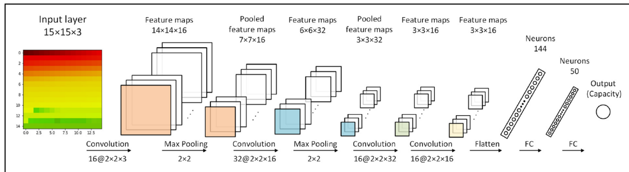
Figure 4. Proposed CNN architecture with 15 \times 15 \times 3 inputs for battery capacity estimation.
