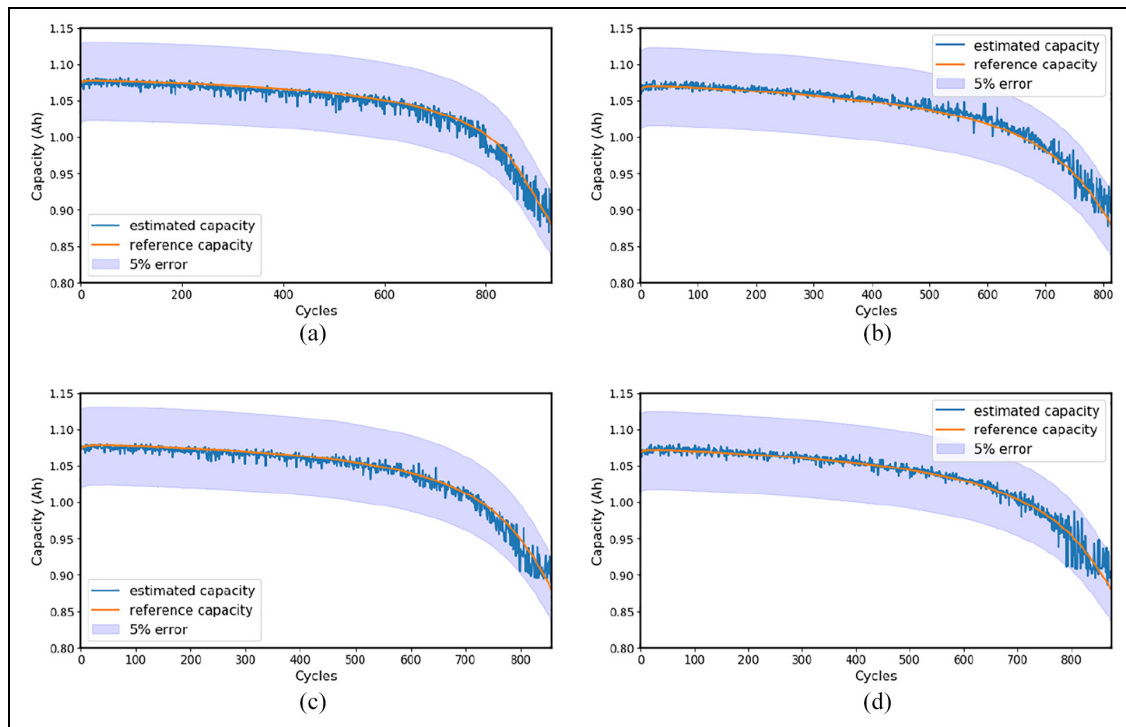
Figure 8. Capacity estimation results on Group 4 (Group 1, 2, 3 for training, and Group 4 for testing). (a) Group 4 – Battery 13 (b) Group 4 – Battery 14 (c) Group 4 – Battery 15 (d) Group 4 – Battery 16.
