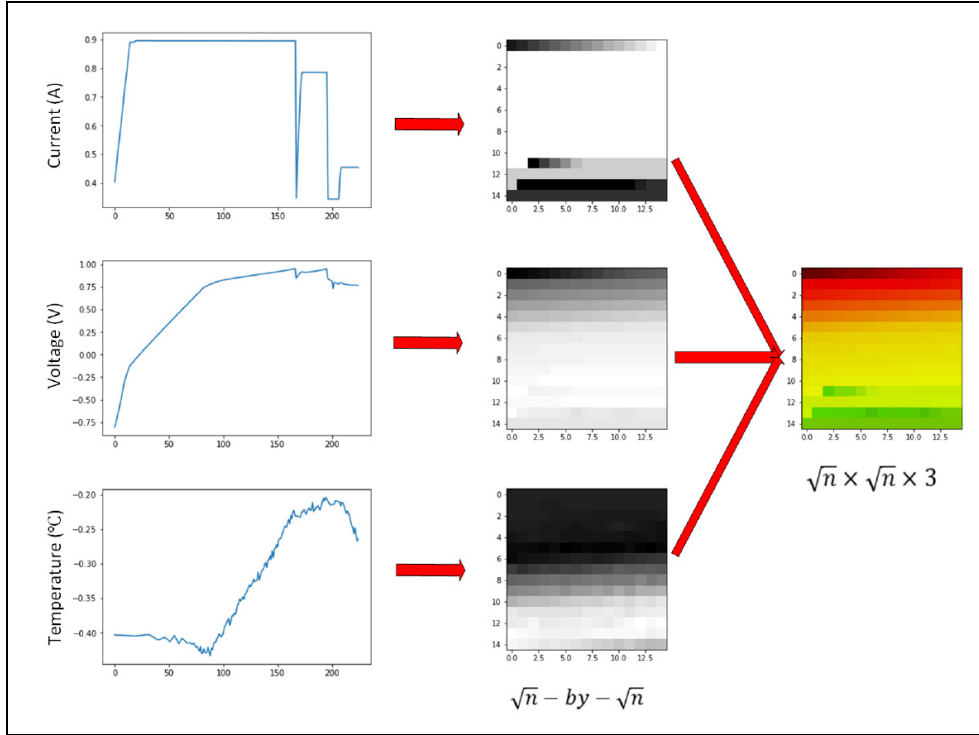
Figure 3. The input of the proposed CNN.
