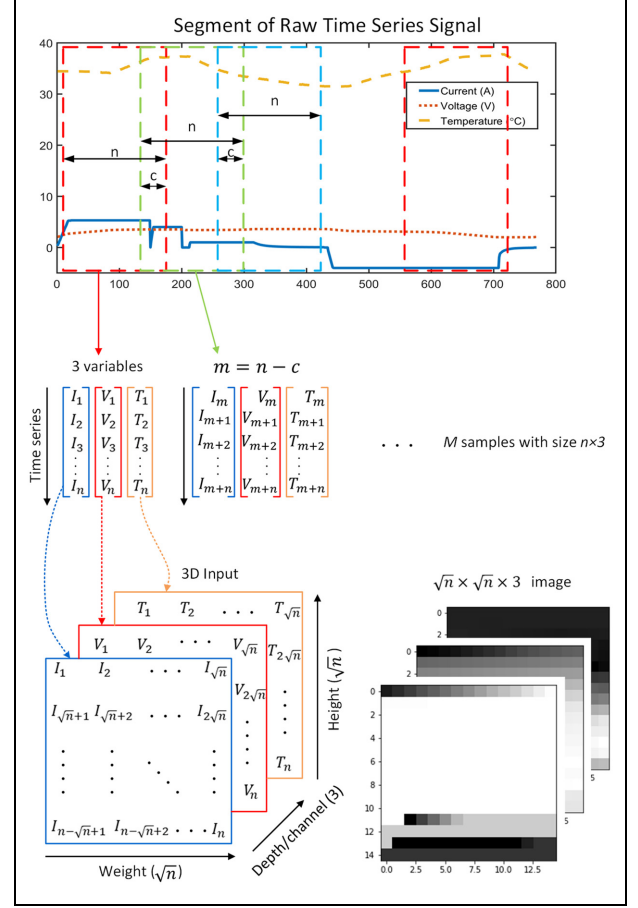
Figure 2. Transformation method: convert the time series measurements to 3-D images.
