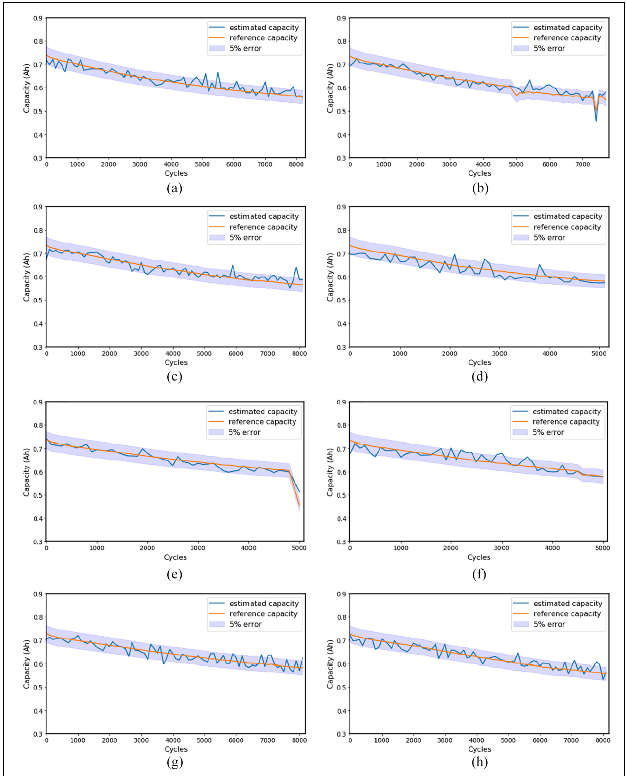
Figure 9. Capacity estimation results of Cell 1 to Cell8.
