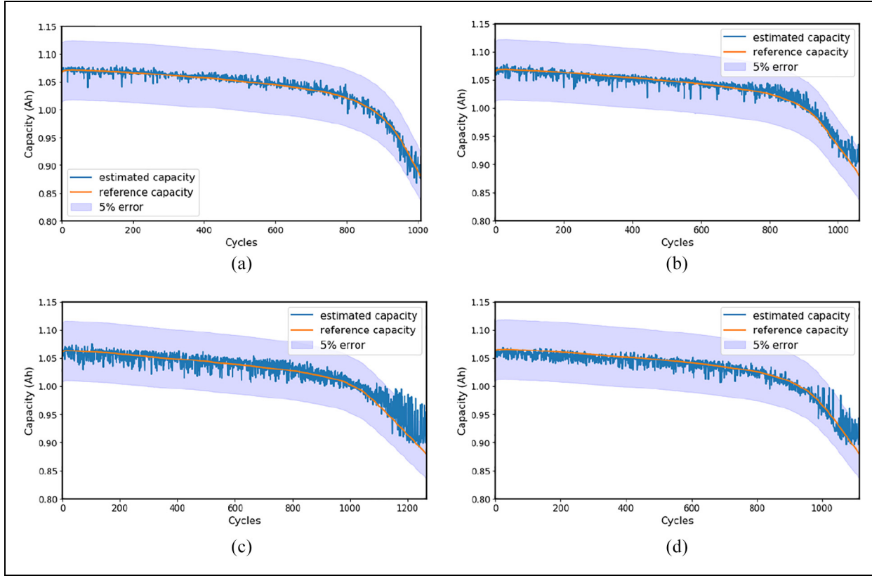
Figure 5. Capacity estimation results on Group I (Group 2, 3, 4 for training, and Group I for testing). (a) Group I – Battery 1 (b) Group I – Battery 2 (c) Group I – Battery 3 (d) Group I – Battery 4.
