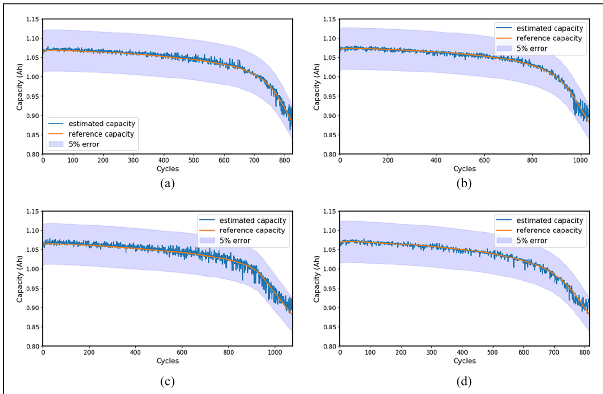
Figure 7. Capacity estimation results on Group 3 (Group 1, 2, 4 for training, and Group 3 for testing). (a) Group 3 – Battery 9 (b) Group 3 – Battery 10 (c) Group 3 – Battery 11 (d) Group 3 – Battery 12.
