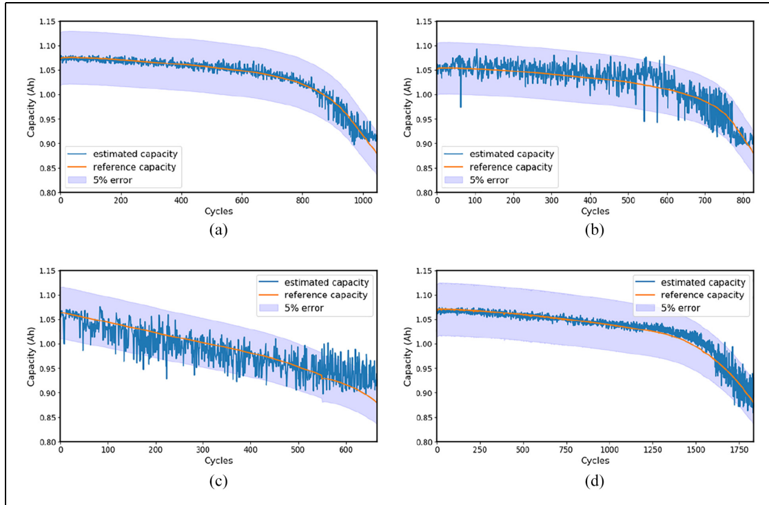
Figure 6. Capacity estimation results on Group 2 (Group 1, 3, 4 for training, and Group 2 for testing). (a) Group 2 – Battery 5 (b) Group 2 – Battery 6 (c) Group 2 – Battery 7 (d) Group 2 – Battery 8.
