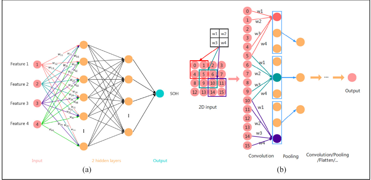
Figure 1. (A) A fully connected three-layer feedforward neural network. (B) A CNN, with convolutional layer as the first layer and pooling layer as the second layer. Here, the filter size is 2 \times 2 with stride (1, 1) , and the pooling size is 1 \times 3 with stride (1, 1) .
