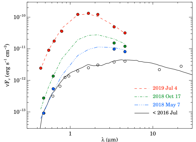
Figure 6. Multiepoch SEDs of Gaia18dvy: quiescence (black circles), peak of the outburst (red dots), and two epochs representing the brightening phase (blue and green dots). The black curve is our best-fitting RADMC3D model to the quiescent measurements, while the other curves are our best-fitting accretion disk models in excess of the quiescent SED.
