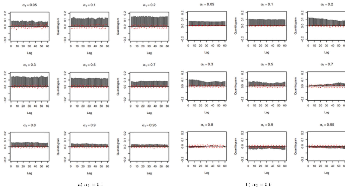
Fig. 18. Cross-quantilogram representing directional predictability from Gold returns to Bitcoin returns. (For interpretation of the references to colour in this figure legend, the reader is referred to the web version of this article.) Source: To detect directional predictability from Gold returns to Bitcoin returns, the sample cross quantilogram \hat{p}_\alpha(k) for \alpha_2 = 0.1 and \hat{p}_\alpha(k) for \alpha_2 = 0.9 . The bar graphs explain sample cross quantilograms, and the lines are the 95% bootstrap confidence intervals.
