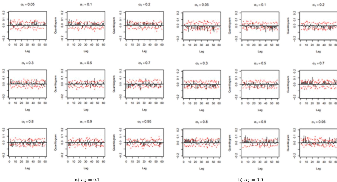
Fig. 5. Cross-quantilogram representing directional predictability from Bitcoin returns to Monero returns. Source: To detect directional predictability from Bitcoin returns to Monero returns, the sample cross quantilogram \hat{p}_\alpha(k) for \alpha_2 = 0.1 and \hat{p}_\alpha(k) for \alpha_2 = 0.9 . The bar graphs explain sample cross quantilograms, and the lines are the 95% bootstrap confidence intervals.
