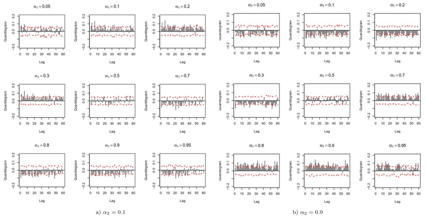
Fig. 11. Cross-quantilogram representing directional predictability from Litecoin returns to Bitcoin returns. Source: To detect directional predictability from Litecoin returns to Bitcoin returns, the sample cross quantilogram \hat{p}_\alpha(k) for \alpha_2 = 0.1 and \hat{p}_\alpha(k) for \alpha_2 = 0.9 . The bar graphs explain sample cross quantilograms, and the lines are the 95% bootstrap confidence intervals.
