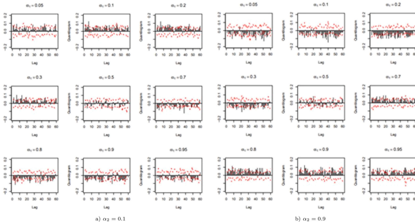
Fig. 3. Cross-quantilogram representing directional predictability from Bitcoin returns to Stellar returns. Source: To detect directional predictability from Bitcoin returns to Stellar returns, the sample cross quantilogram \hat{p}_\alpha(k) for \alpha_2 = 0.1 and \hat{p}_\alpha(k) for \alpha_2 = 0.9 . The bar graphs explain sample cross quantilograms, and the lines are the 95% bootstrap confidence intervals.
