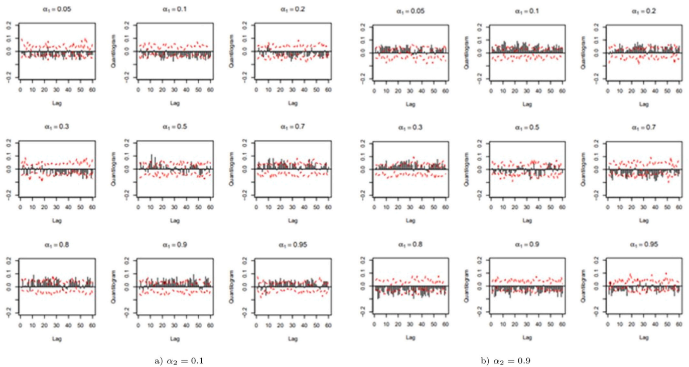
Fig. 19. Cross-quantilogram representing directional predictability from Oil returns to Bitcoin returns. Source: To detect directional predictability from Oil returns to Bitcoin returns, the sample cross quantilogram \hat{P}_\alpha(k) for \alpha_2 = 0.1 and \hat{P}_\alpha(k) for \alpha_2 = 0.9 . The bar graphs explain sample cross quantilograms, and the lines are the 95% bootstrap confidence intervals.
