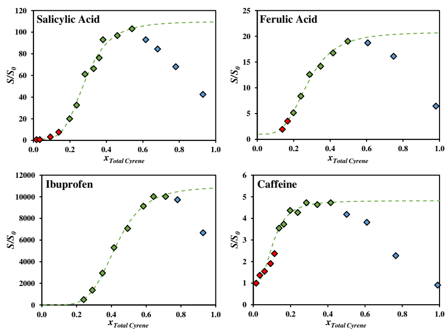
Figure 4. Solubility increase ( S/S_0 ) of the hydrophobic solute as a function of total Cyrene mole fraction ( \blacklozenge, \blacktriangle, \blacklozenge ), along with the fitting curves of the cooperative model using only the green data points (green dashed line). Data by De bruyn et al. 14
