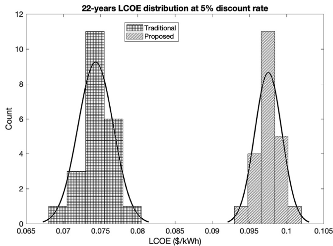
Fig. 10. LCOEs for PV with traditional and proposed methods.
