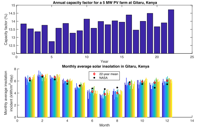
Fig. 9. The monthly average solar insolation and annual CF at a solar PV farm in Gitaru, Kenya.
