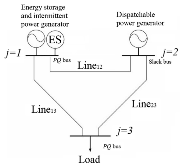
Fig. 8. A 3-bus system with two generators and a load.
