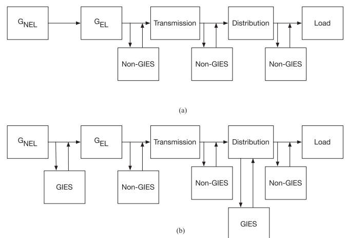
Fig. 2. An electrical power system consisting of a) Non-GIES only; b) GIES and non-GIES.
