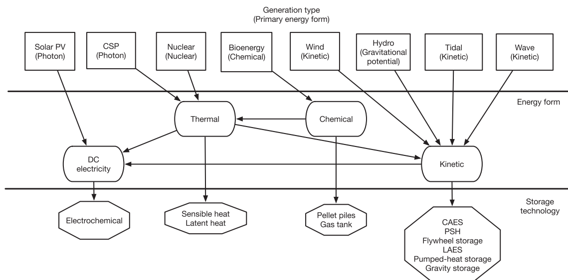
Fig. 1. Energy transformation processes between low-carbon power generation and possible generation-integrated energy storage technologies.
