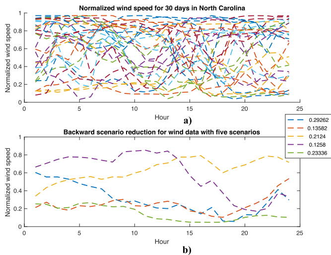
Fig. 4. a) The normalized wind speed for 30 days in North Carolina, USA; b) the five reduced scenarios, data from (NREL Wind Prospector).
