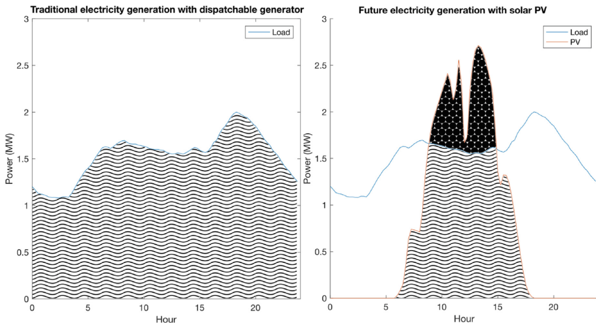
Fig. 6. a) Load met with dispatchable generators in a traditional electrical power system; b) Load met with PV plant in a future system.
