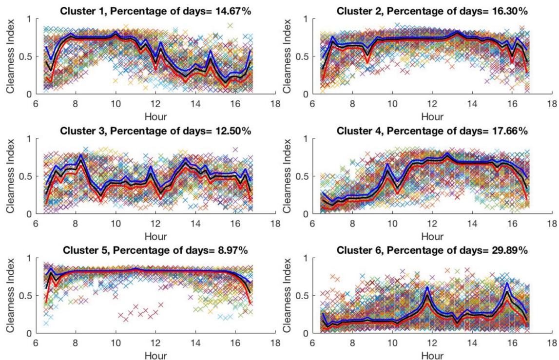
Fig. 5. Scenario reduction for solar clearness index in Kenya during winter with Fuzzy C-means and Dynamic Time Warping (Lai, 2017).
