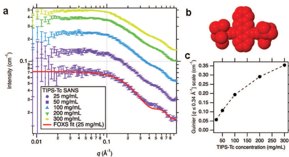
Fig. 2 (a) Small-angle neutron scattering (SANS) of TIPS-Tc in deuterated toluene at concentrations ranging from 25 to 300 \text{mg mL}^{-1} , with the associated fit to an X-ray scattering model of TIPS-Tc in \text{H}_2\text{O} (using the FOXS 34,35 server), to confirm the molecule's overall shape only (b) representation of TIPS-Tc shape used by FOXS to calculate the molecular scattering, rendered using an implementation of Jmol/JSmol. 36 (c) The scale factor of the Guinier fit to the SANS data in the range q = 0.008\text{--}0.34 \text{\AA}^{-1} indicative of the relative volume fractions of TIPS-Tc, as a function of nominal TIPS-Tc concentration.
