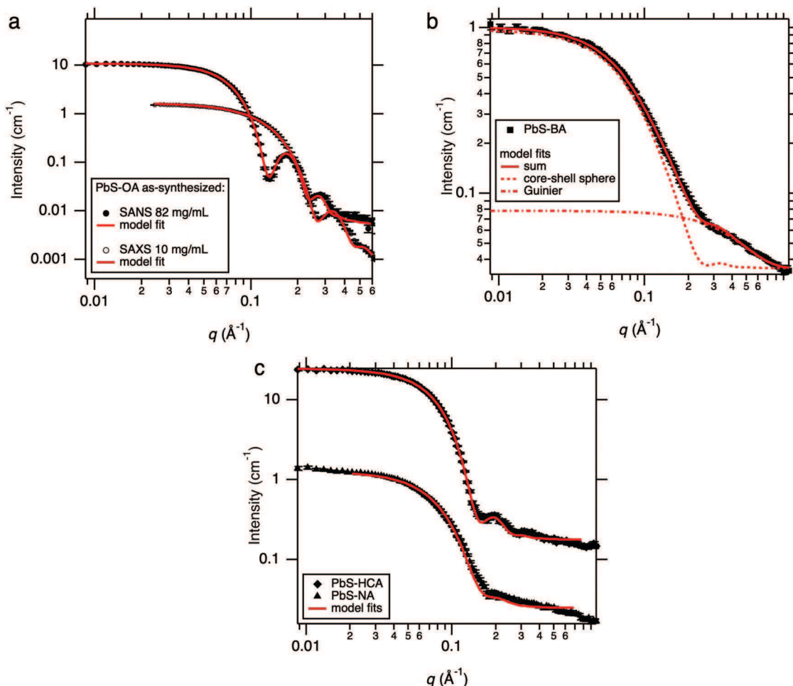
Fig. 1 (a) SANS and SAXS from the stock PbS-OA at respective concentrations of 82 \text{mg mL}^{-1} and 10 \text{mg mL}^{-1} (see also ref. 21) along with model fits from a core-shell sphere * hard sphere model and a sphere * hard sphere model respectively (b) SANS from PbS-BA, which implies the presence of smaller ligand complexes in addition to quasi-spherical QDs. (c) SANS from PbS-NA and PbS-HCA with associated core-shell-sphere model fits.
