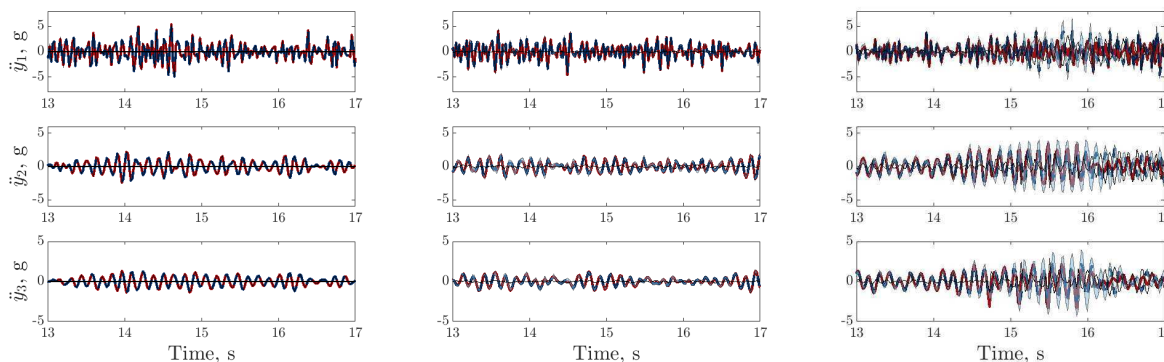
Figure 7. Digital twin \mathcal{M}^{GP}(\{\mathcal{M}^l(F, \theta_{\mathcal{D}_1}^{MAP}), F\}, \hat{\phi}_{\mathcal{D}_1}) predictions, trained using dataset one \mathcal{D}_1 , between 13 and 17s on datasets one to three (left to right); measured acceleration \{\ddot{y}_i\}_{i=1}^3 (—), digital twin mean prediction (---), digital twin \pm 3\sigma confidence intervals (blue shaded region), residual error (—).
