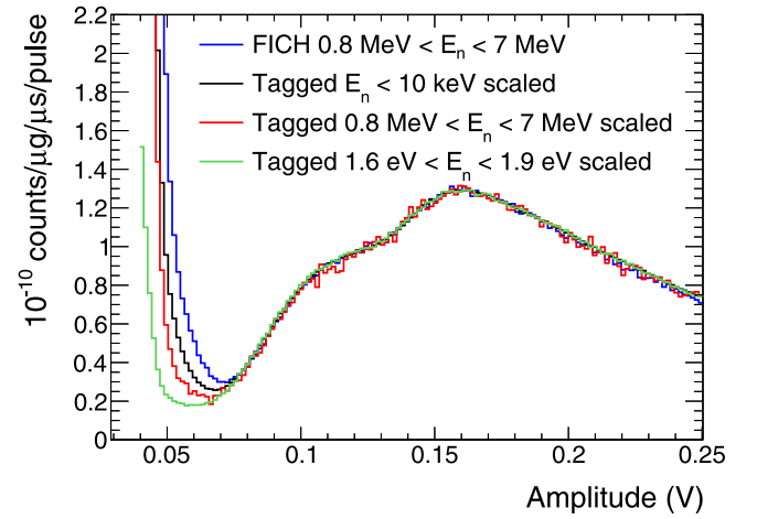
Fig. 17. Pulse height spectra of the events in the fission chamber for 0.8 \text{ MeV} < E_n < 7 \text{ MeV} compared to tagged events for different E_n regions from all FICH channels. The neutron flux of n_{TOF} can be seen in Fig. 7.
