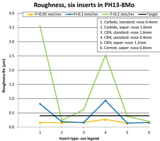
Fig. 4. Roughness R_a for six different inserts at three feed rates on PH13-8Mo steel. Surface speed 150 m/min for inserts 1 and 2, 230 m/min for inserts 3, 4 and 5 and 180 m/min for insert 6. Speeds recommended by tool manufacturer.
