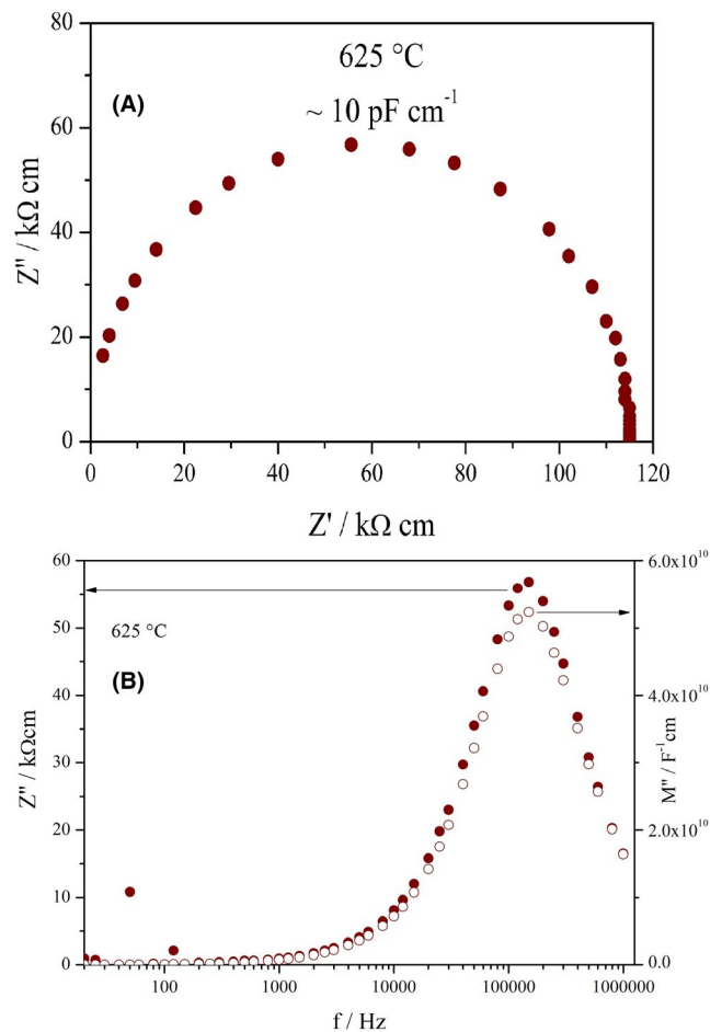
FIGURE 9 Typical impedance spectroscopy data collected for Pss07 at 625°C. (A) Complex impedance plot and (B) combined spectroscopic plots of the imaginary components of impedance and electric modulus
