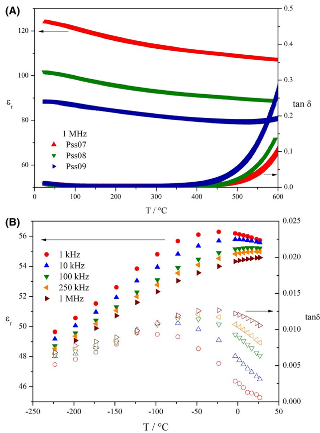
FIGURE 8 A, Temperature profiles of permittivity and dielectric loss for Pss ceramics (~95% relative density) at 1 MHz. B, Subambient temperature profiles of the permittivity and dielectric loss for Pss10 (~75% relative density)
