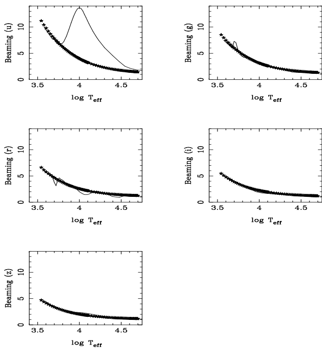
Fig. 1: Comparison between the beaming factors according to Eq. (3) (HiPERCAM passbands). The DA white dwarf models are represented by continuous lines and black body approximation by stars. All models are at \log g = 5.0 .
