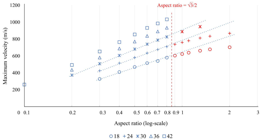
Figure 24: Graph of maximum velocity versus charge aspect ratio (log scale), grouped by charge diameter.
