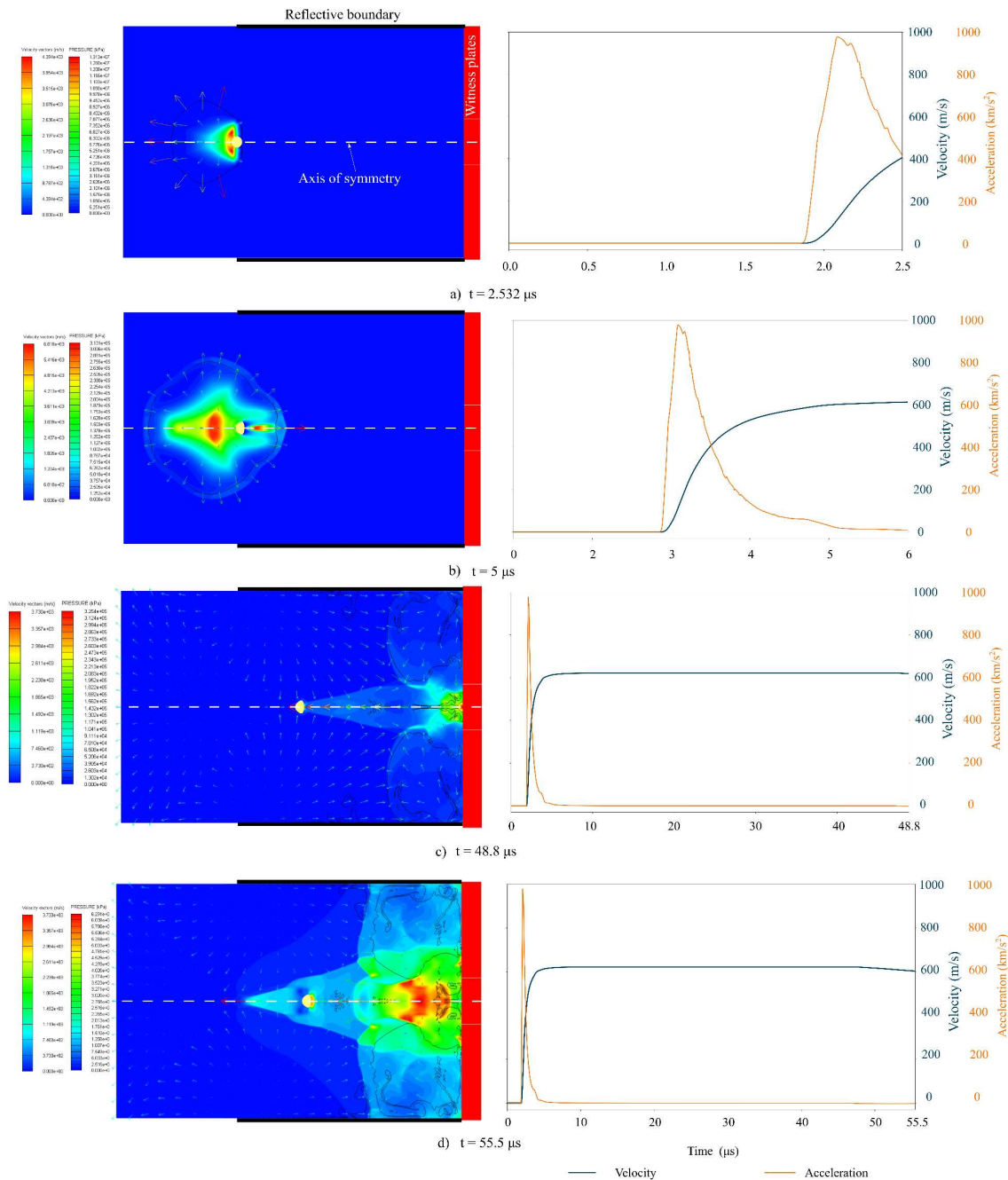
Figure 22: Simulated pressure contours, velocity vectors (left), velocity and acceleration histories (right) at different times experienced by a typical ball bearing for a \text{Ø} 18 \text{ mm} , L/D=1 detonation.
