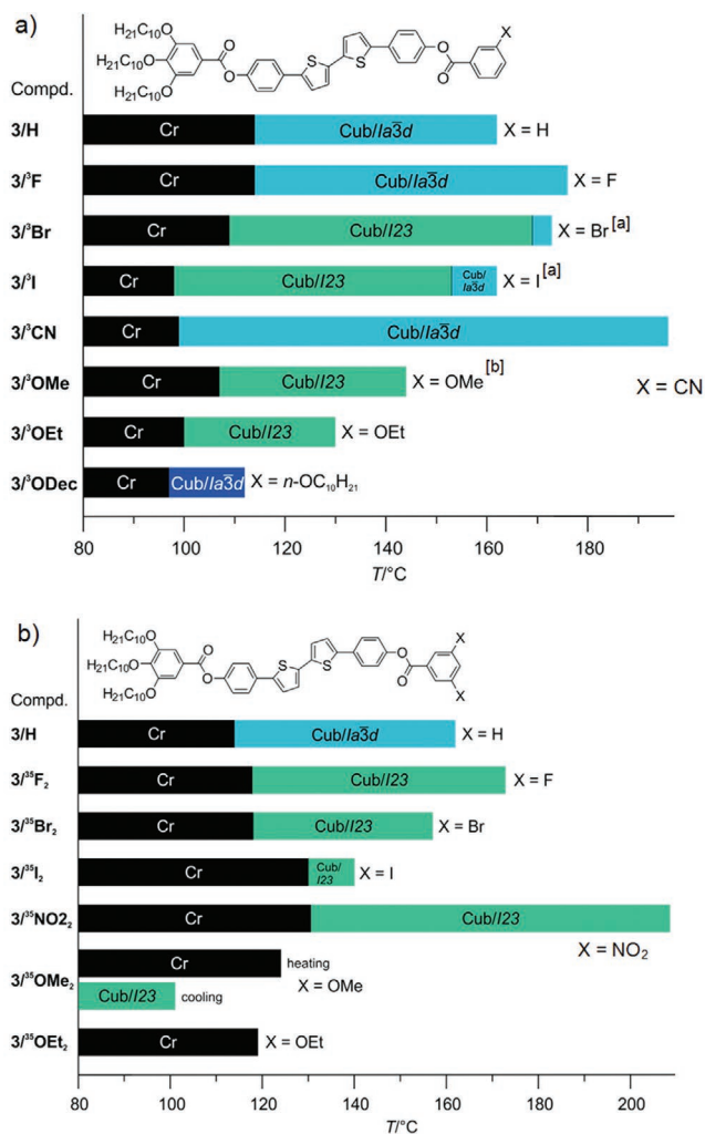
Figure 4. Mesophases and transition temperatures a) of compounds 3/3^X and b) of compounds 3/3^{5X_2} , recorded on heating; for compound 3/3^{\text{ODec}} , a \text{Col}_{\text{hex}} phase is formed on cooling from Iso which is rapidly replaced by the Ia\bar{3}d phase (see Figure S2 in the Supporting Information); the Ia\bar{3}d phase of 3/3^{\text{ODec}} , indicated by a darker blue, represents a short pitch Ia\bar{3}d_{(S)} phase, whereas all others, shown in light blue belong to the long pitch Ia\bar{3}d_{(L)} type. [a] For 3/3^{\text{Br}} and 3/3^{\text{I}} only, the Ia\bar{3}d phase is observed on cooling; [b] for 3/3^{\text{OMe}} on cooling, Ia\bar{3}d and I23 phases were observed, depending on the condition, see Section S1.4 in the Supporting Information; the numerical data are collated in Table S1 in the Supporting Information and for 3/3^{\text{H}} and 3/3^{\text{OEt}} , see ref. [87].
