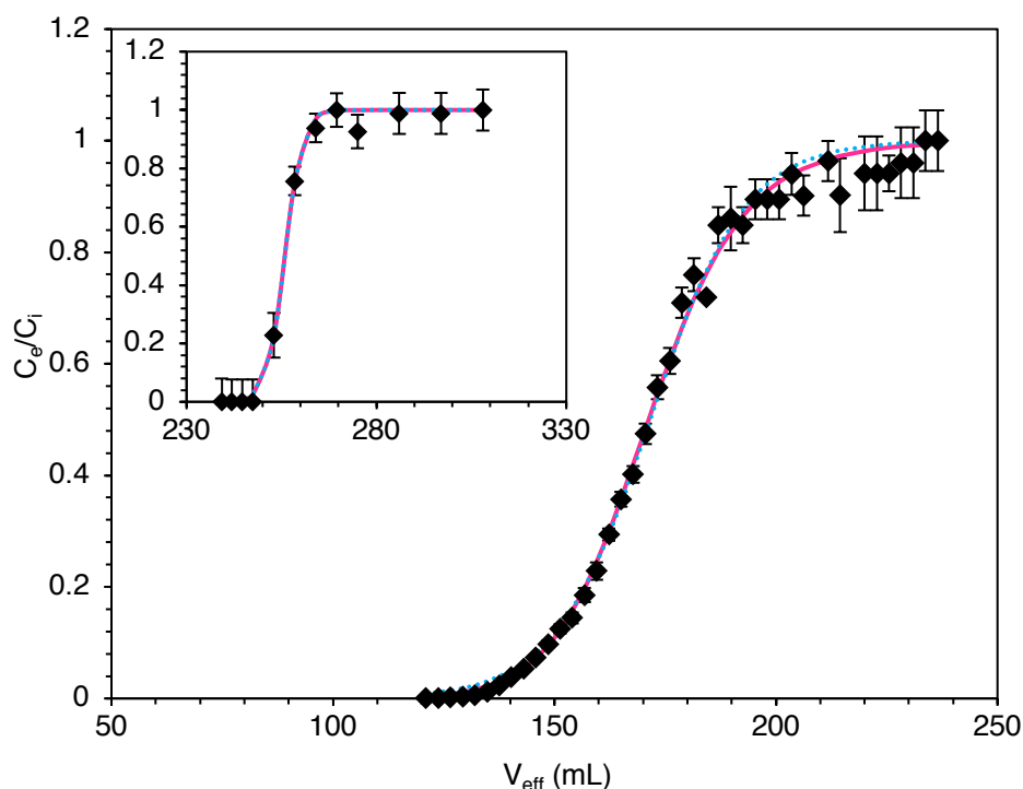
Figure 6. Breakthrough curves for M4195-Cu with iodide, 10 meq nitrate and 10 meq molybdate solution, fitted to the Dose-Response (pink line) and Adams-Bohart (dotted blue line) dynamic models.. Main image shows initial breakthrough. Inset shows 2 nd breakthrough. Resin BV = 5.50 mL. Inlet [I - ] = 2.00 g.L -1 . Flow rate = 1 BV.hr -1 . T = 20°C. Error bars represent the approximate 95 % confidence intervals, derived from 3 x electrode measurements.
