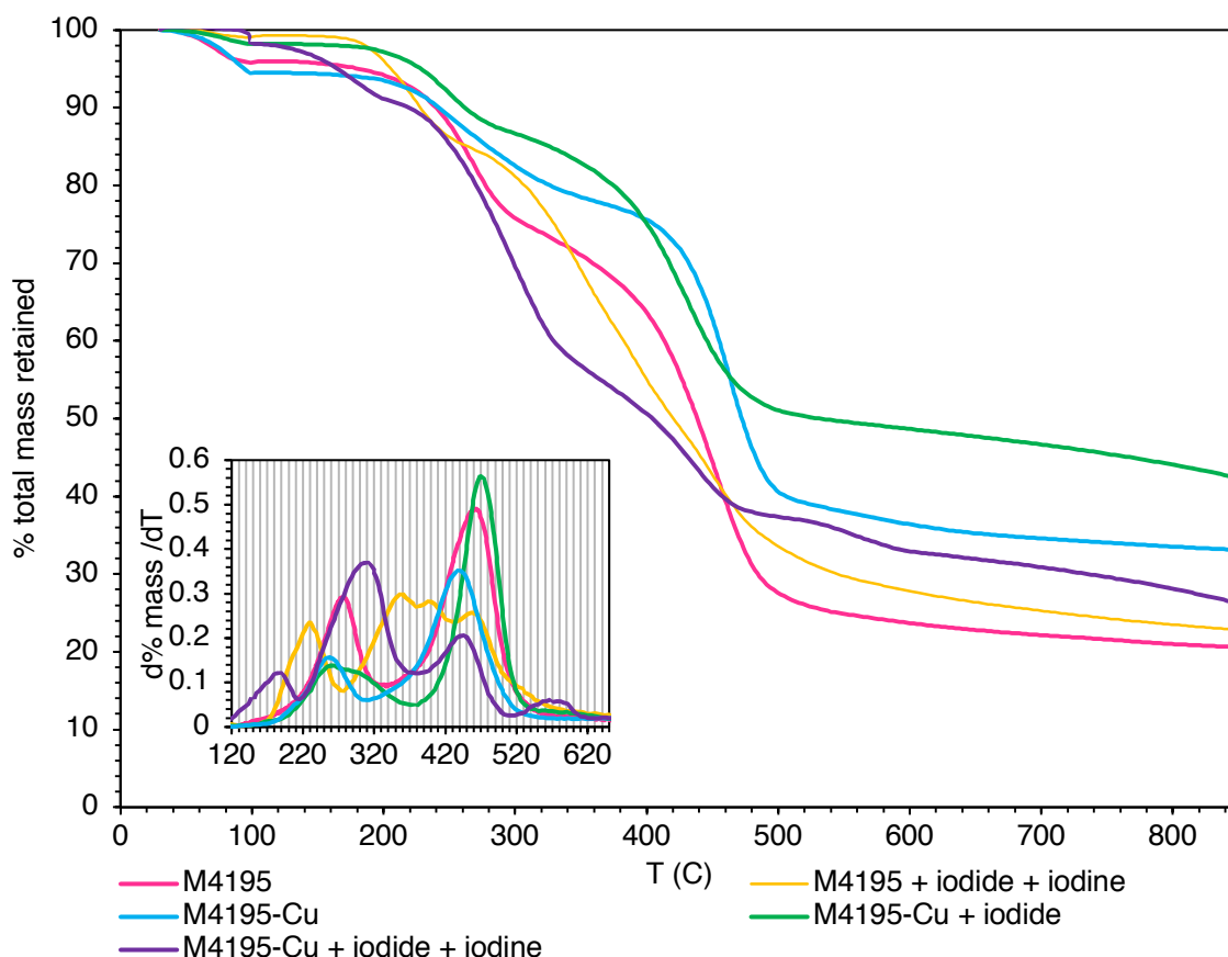
Figure 8. Thermograms of M4195 resin samples at various processing stages, in oxidising conditions. Inset shows first derivative. For samples contacted with solutions of iodine species, initial [I^-] = 1000 \text{ mg.L}^{-1} . Initial [I_2] = 1000 \text{ mg.L}^{-1} .
