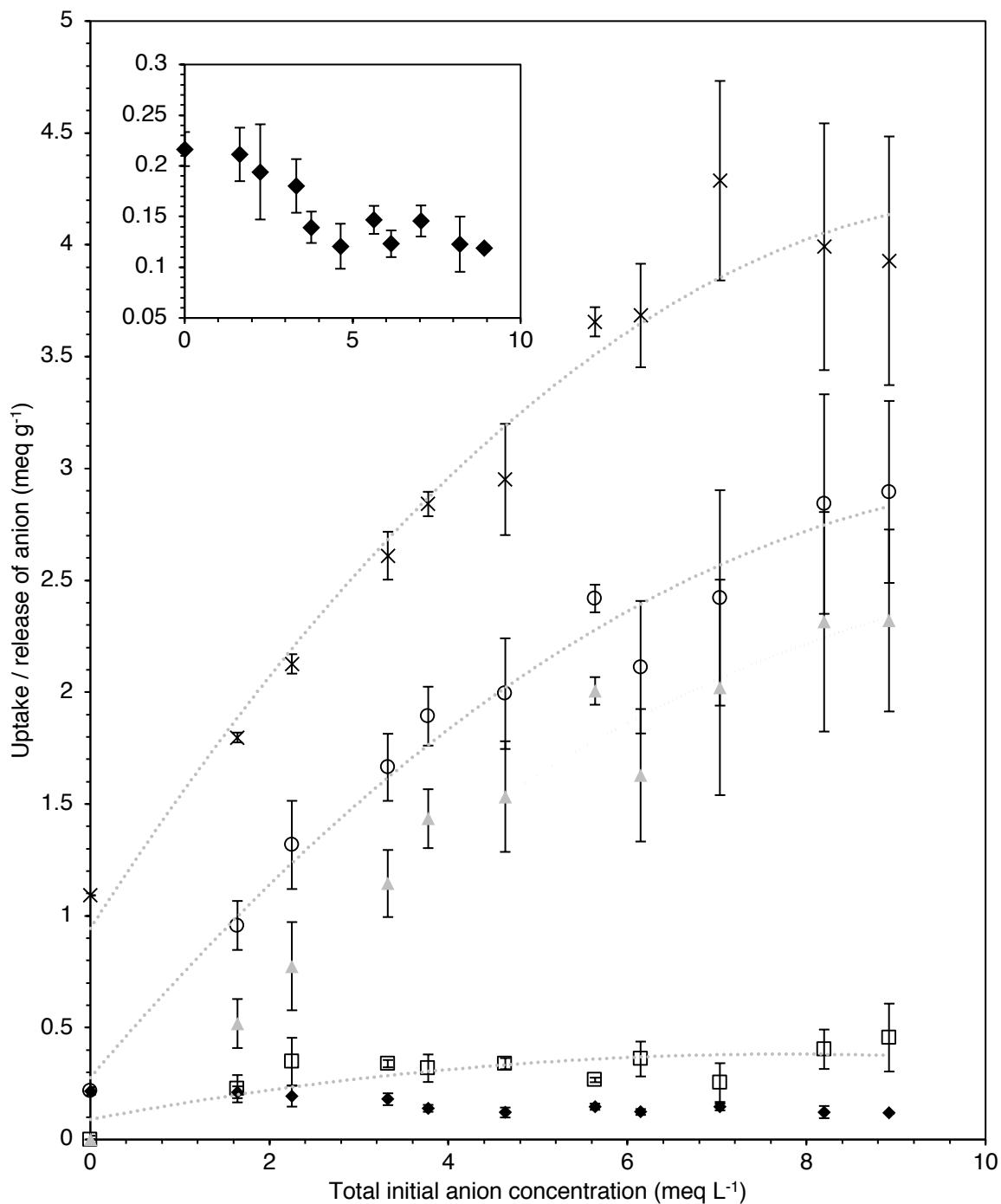
Figure 3. Uptake of iodide (◆), nitrate (□), molybdate (▲) and total anions (○), with accompanying release of chloride (×) in mixed anions systems. 2 nd order polynomial fits added to guide the eye. Inset shows enlargement of iodide uptake data. Initial [I - ] = 50 mg.L -1 . Cocontaminant molar ratio = 0-10. Solution volume = 50.0 mL. Sorbent mass = 100 mg. Contact time = 24 hr. T = 20°C. Error bars represent approximate 95 % confidence intervals derived from 2 x experimental reps.
