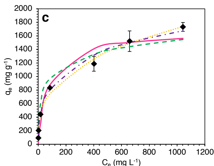
Figure 2. Uptake isotherms of iodine species on to M4195-Cu with fitting to common thermodynamic models. (a) Iodide only system. (b) Iodide uptake only from mixed iodide/iodine system. (c) Total iodine uptake from mixed iodide/iodine system. Initial [I^-] = 50\text{--}2000\text{ mg}\cdot\text{L}^{-1} . Initial [I_2] = 300\text{--}6000\text{ mg}\cdot\text{L}^{-1} . Solution volume = 50.0 mL. Sorbent mass = 100 mg. Contact time = 24 hr. T = 20^\circ\text{C} . Error bars represent approximate 95 % confidence intervals derived from 2 x experimental reps.
