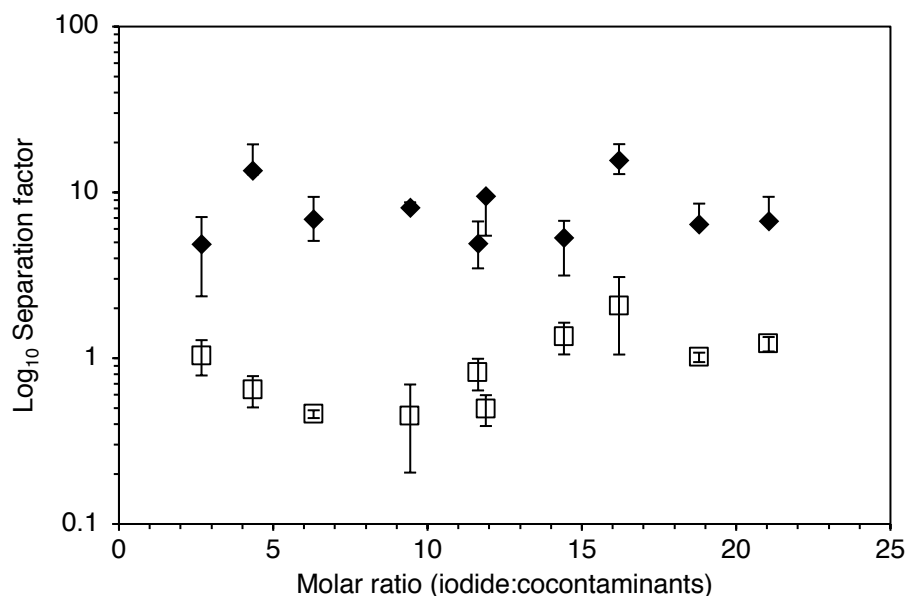
Figure 4. Determined separation factors (S.F.s) for iodide versus nitrate (◆) and molybdate (□). All experimental conditions as per Figure 3.
