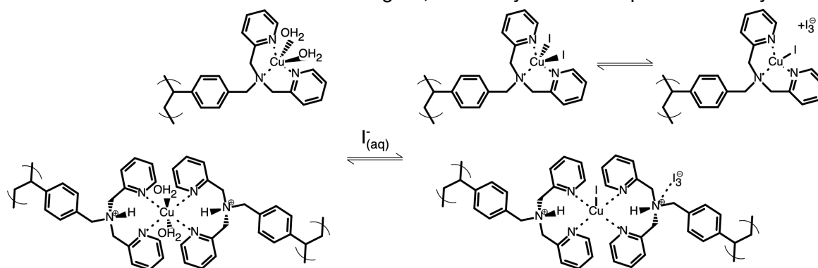
Scheme 2. Proposed loading mechanisms of iodide on to M4195-Cu.
