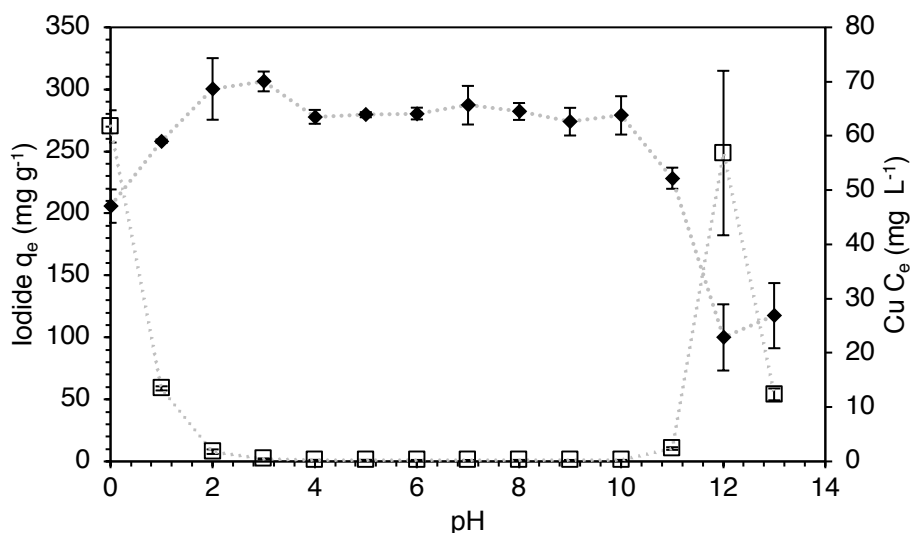
Figure 1. Iodide uptake of M4195-Cu over pH range 0 - 13 with adjustments being made using HNO 3 and NaOH. Solution volume = 5 mL. Initial [I - ] = 1.00 g.L -1 . Equilibration time = 24 hr. Resin mass = 100 mg. T = 20°C. Error bars represent approximate 95 % confidence intervals derived from 2 x experimental reps.
