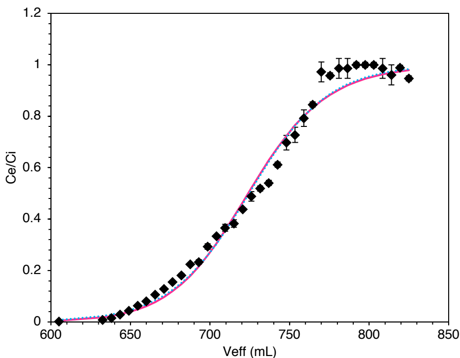
Figure 5. Breakthrough curve for M4195-Cu with an iodide only solution, fitted to the Dose-Response (pink line) and Adams-Bohart (dotted blue line) dynamic models. Resin BV = 5.50 mL. Inlet [I^-] = 2.00 g.L -1 . Flow rate = 1 BV.hr -1 . T = 20°C. Error bars represent the approximate 95% confidence intervals, derived from 3 x electrode measurements.
