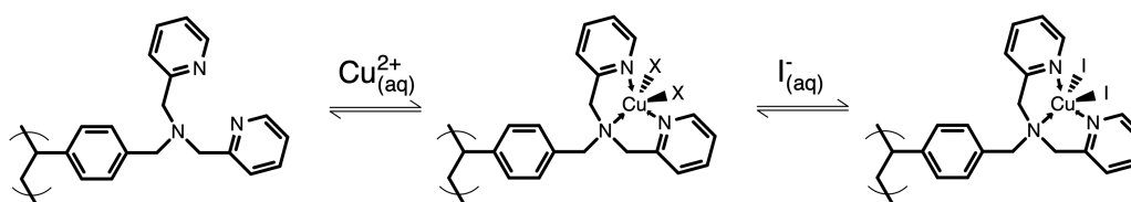
Scheme 1. Proposed metallation and iodide uptake of M4195 resin.
