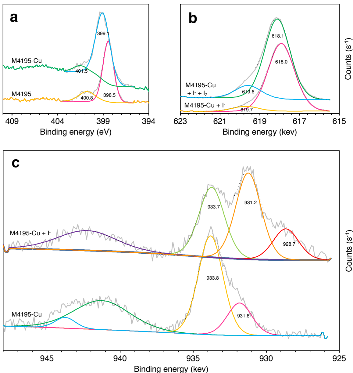
Figure 7. Selected high resolution XPS spectra of M4195 resin, at various processing stages: (a) N 1s, (b) I 3d, (c) Cu 2p 5/2. For samples contacted with solutions of iodine species, initial [I^-] = 1000 \text{ mg}\cdot\text{L}^{-1} . Initial [I_2] = 6000 \text{ mg}\cdot\text{L}^{-1} .
