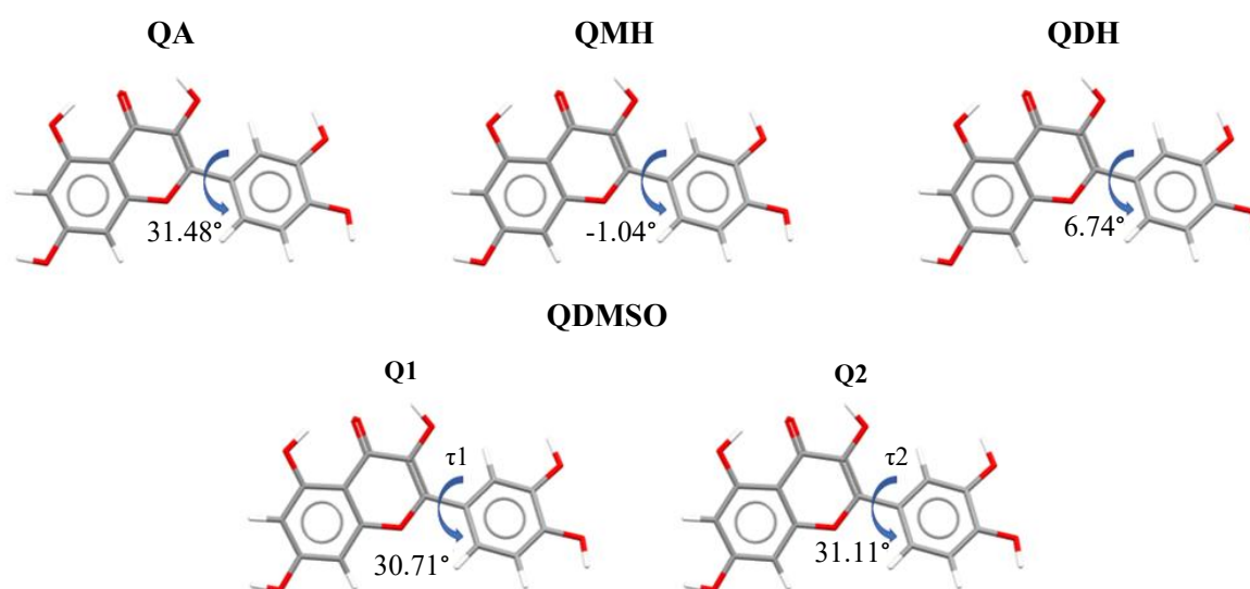
9 10 Figure 4. Torsion angles of phenyl to pyrone rings for quercetin molecules in quercetin 11 structures (quercetin anhydrous – QA, quercetin monohydrate – QMH, quercetin dihydrate – 12 QDH, quercetin – DMSO solvate – QDMSO). 22
