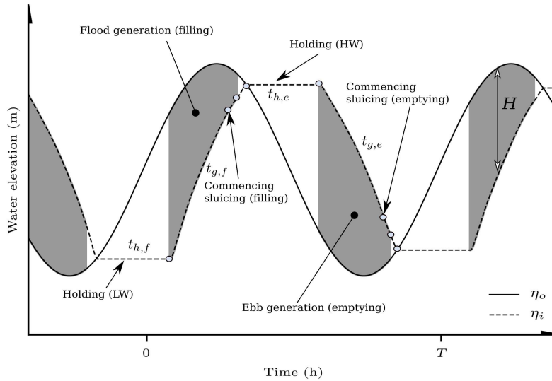
Figure 3: Two-way operation schematic for a conventional tidal power plant over an M2 tidal period T = 12.42\text{h} , illustrating typical modes of operation. The grey shaded areas indicate periods when power is generated. t_{h,e}, t_{h,f}, t_{g,e}, t_{g,f} comprise operational controls used in the algorithm presented in Angeloudis et al. (2018) for a two-way operation sequence. For the generic “fixed-control” (Harcourt et al., 2019) operation these were set to t_{h,e} = t_{h,f} = 3.25\text{h} t_{g,e} = t_{g,f} = 3.0\text{h} respectively.
