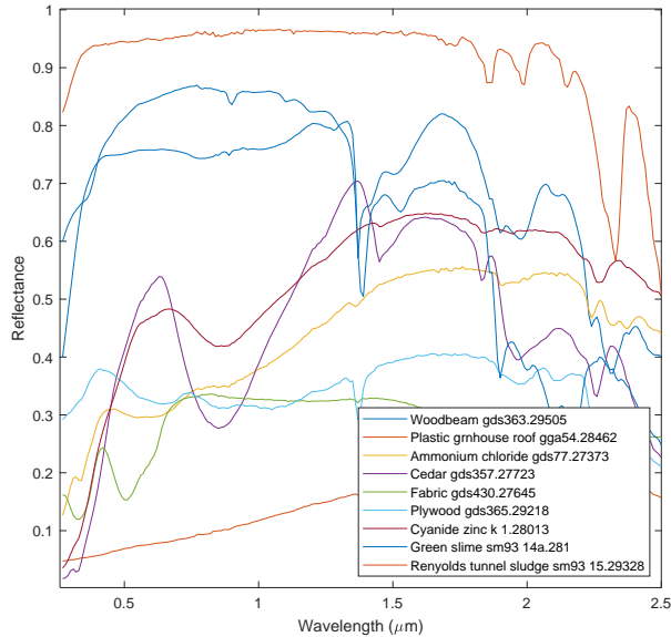
Fig. 2. The spectral curve of the 9 endmembers selected from the USGS mineral spectra library on the simulated datasets.
