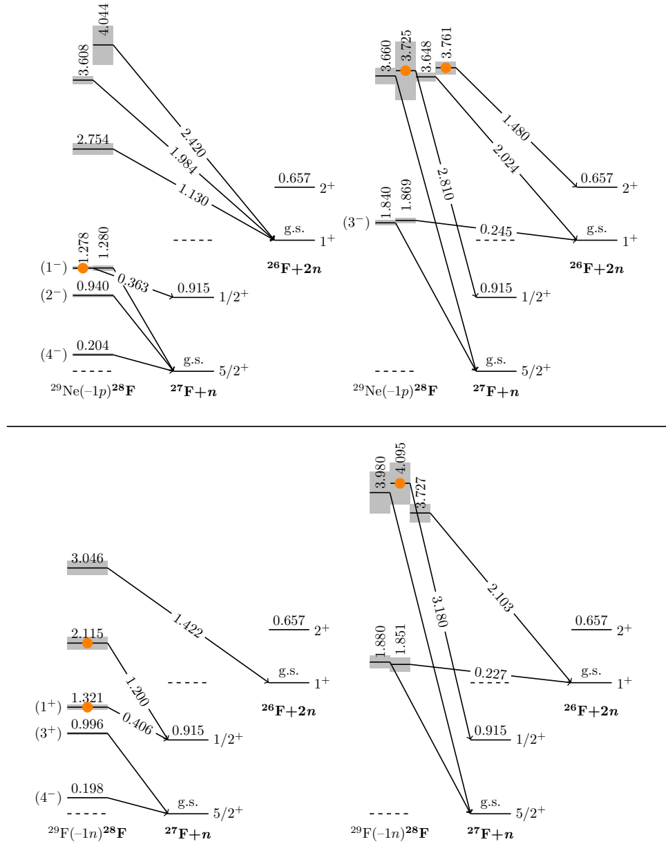
FIG. S1: The detailed decay scheme of the different states observed in ^{28}\text{F} , populated from ^{29}\text{Ne} and ^{29}\text{F} , is shown in the top and bottom panels, respectively. The widths of the levels correspond to the uncertainty on their centroid value, while the placement of the levels marked with a filled orange circle is derived from their observed coincidence with a \gamma -ray in the ^{27}\text{F} or ^{26}\text{F} spectra from the 1n or 2n emission, respectively. The level scheme of ^{28}\text{F} has been divided into two regions (left and right) for better clarity.
