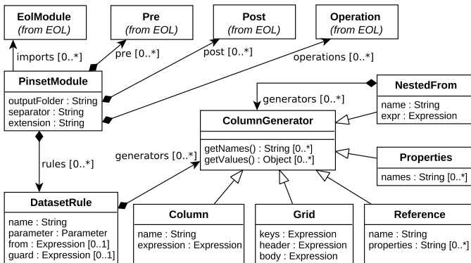
Fig. 3. Abstract syntax of Pinset.
