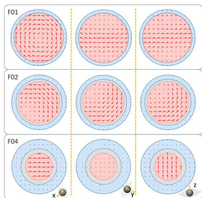
Figure 8. (A) Cross sections of magnetization configurations at remanence for the samples F01, F02, and F04 discussed in Table 2; the magnetization arrows correspond to the average over 8-unit cells. The snapshots have been taken along the X, Y, and Z directions (left, center, and right snapshot for each sample, respectively) and always at the center of the particle.
