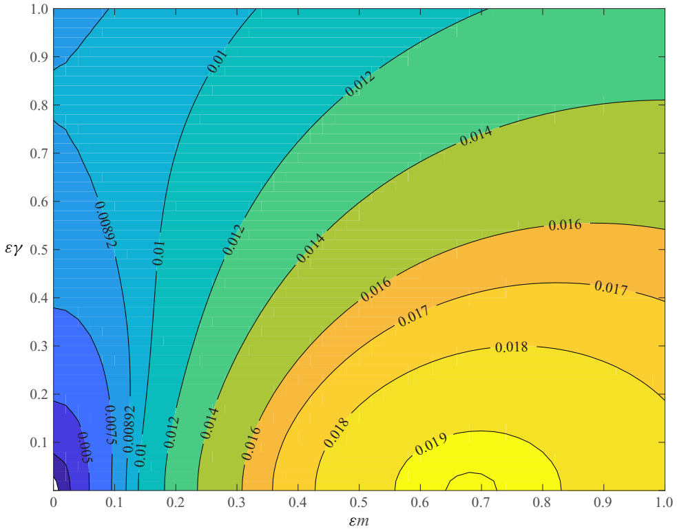
FIGURE 11. A contour of \Lambda(f_\epsilon)/\epsilon over (\epsilon m, \epsilon \gamma) showing that maximum \Lambda(f_\epsilon) is 0.019\epsilon at (\epsilon m, \epsilon \gamma) = (0.68, 0) (data for \epsilon = 0.001 shown).
