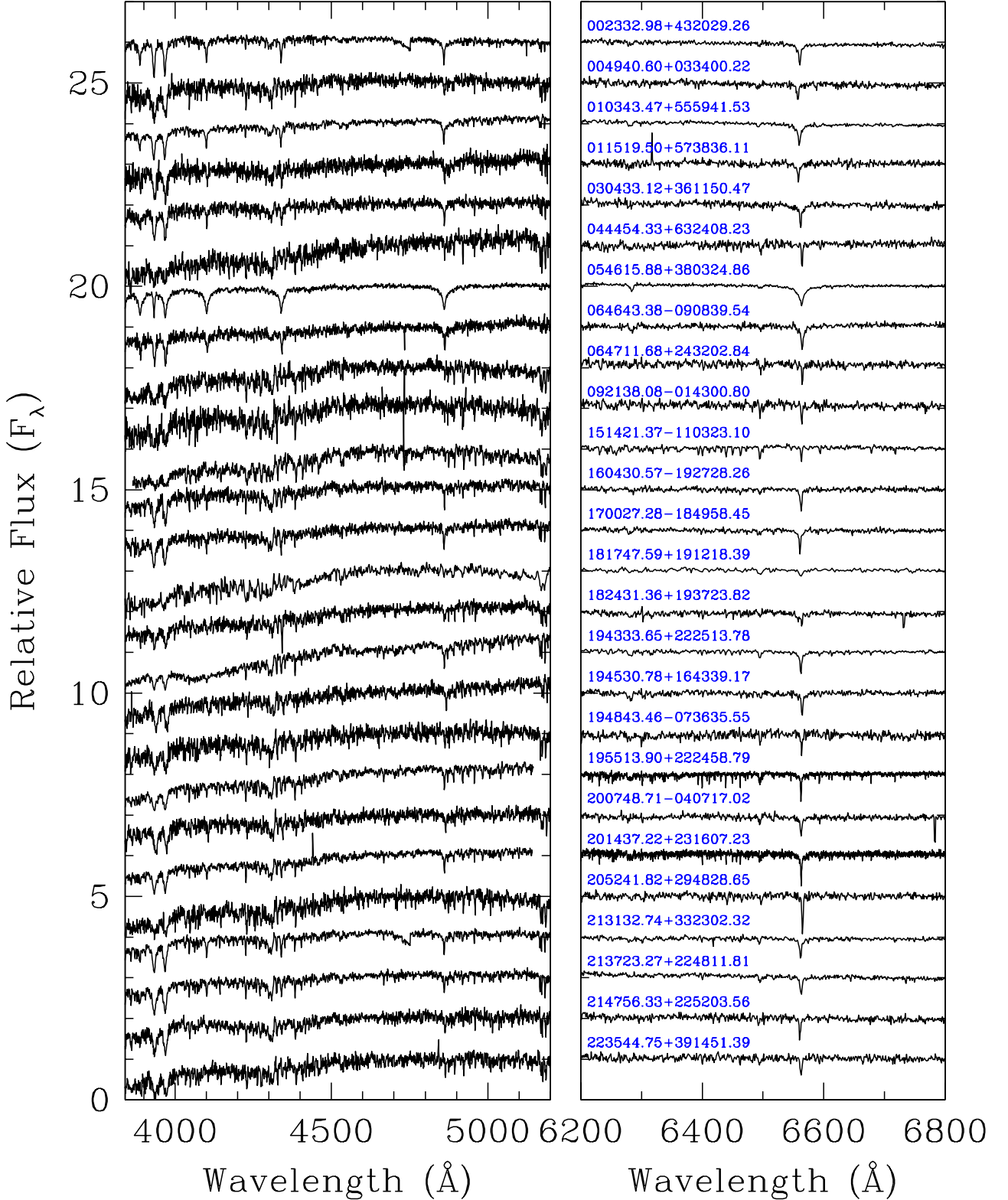
Figure A20. Spectroscopic observations of main-sequence stars that are low-probability white dwarf candidates ( P_{\text{WD}} < 0.75 ) in the catalogue of Gentile Fusillo et al. (2019).
