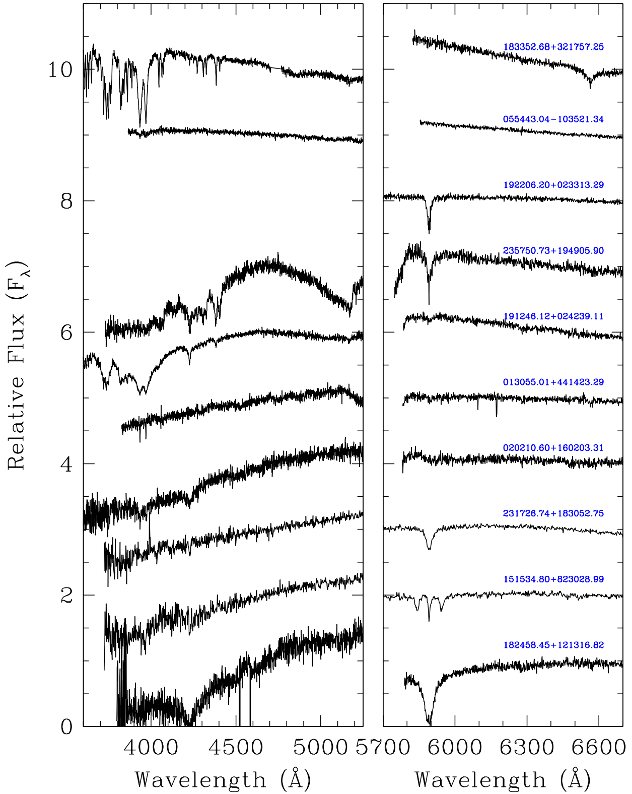
Figure A18. Spectroscopic observations of 10 DZ, DZA and DZH white dwarfs.
