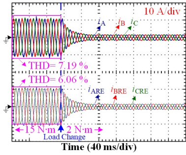
Fig. 11. Waveforms of actual and calculated three-phase currents during load change (All current sensors survive, reconfigured topology).
