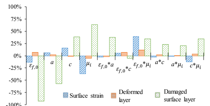
Fig. 7. Influence of the input parameters of the ductile failure model on surface drag.
