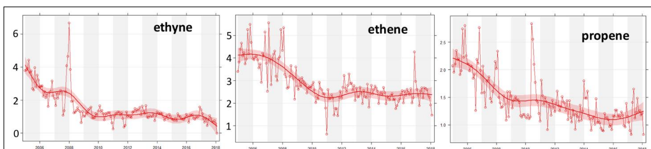
Figure 8. Deseasonalised trends in ethyne, ethene and propene (units \mu\text{g m}^{-3} ) at Marylebone Road 2005-2018. Data from Defra Automated Hydrocarbon network. Solid line is the trend, shaded area 95% confidence interval.
