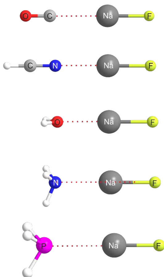
Figure 2. Type I complexes of B\cdots NaF . The geometry of OC\cdots NaF is that at the single minimum detected. For the remaining complexes two minima were detected and the geometries displayed pertain to the higher energy of the two minima.
