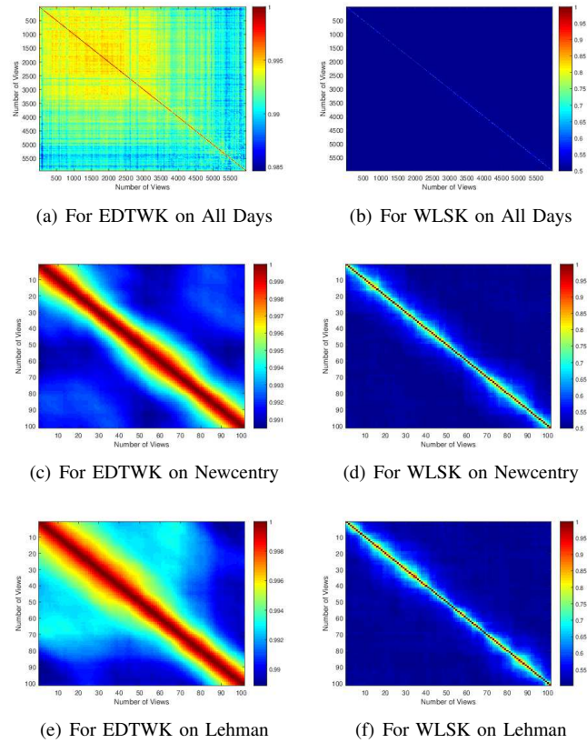
Fig. 11. Kernel Matrices Visualizations for EDTWK and WLSK Kernels.
