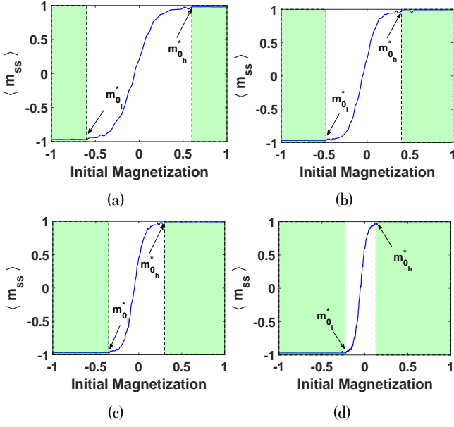
FIG. 2: Dependency of mean steady state magnetization on initial magnetization, (a) N = 50, I_+ = 6, I_- = 5 , (b) N = 100, I_+ = 12, I_- = 10 , (c) N = 200, I_+ = 24, I_- = 20 , (d) N = 500, I_+ = 60, I_- = 50
