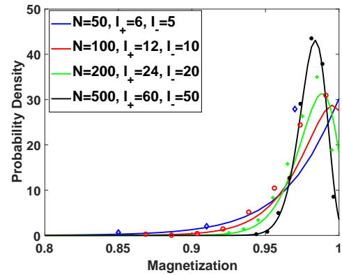
FIG. 1: Effect of the population size N on the steady state density P_{ss}(m)
