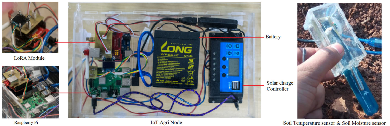
FIGURE 4. IoT Agri Node with its components.
