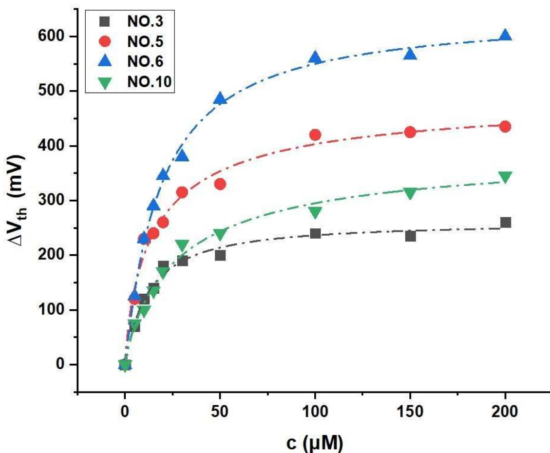
Fig. 3: Threshold shift \Delta V_{th} vs. c in response to waterborne benzyl alcohol for WGTFTs sensitized with zeolites No.s 3, 5, 6, 10. The dashed lines are fits to eq. 1.
