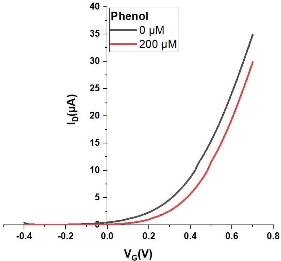
Fig. 4: Linear transfer characteristics for \text{SnO}_2 WGTFTs sensitized with zeolite No. 2 filled plasticized PVC membrane under pure water, and water with high concentration (200 \mu\text{M} ) of phenol.
