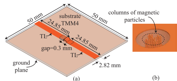
FIGURE 8. (a) Dimensions of a 50 \Omega TL with the MRS modeled in HFSS and (b) magnetic particles modeled as conducting spheres and columns of magnetic particles to show MRS ‘ON’ state.
