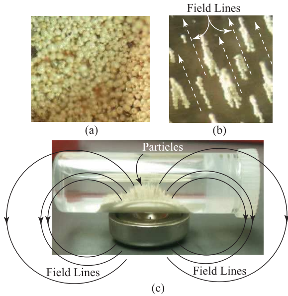
FIGURE 3. (a) Photograph of the particles under a microscope; (b) photograph of the particles columnizing on a flat surface in the direction of the field-lines; and (c) photograph of the particles initially dissolved in alcohol aligning with the field lines.
