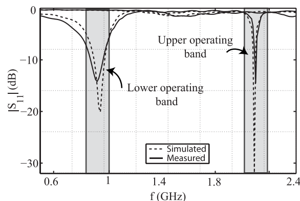
FIGURE 15. Simulated and measured S-parameter of the EBG antenna embedded with novel MRSs.
